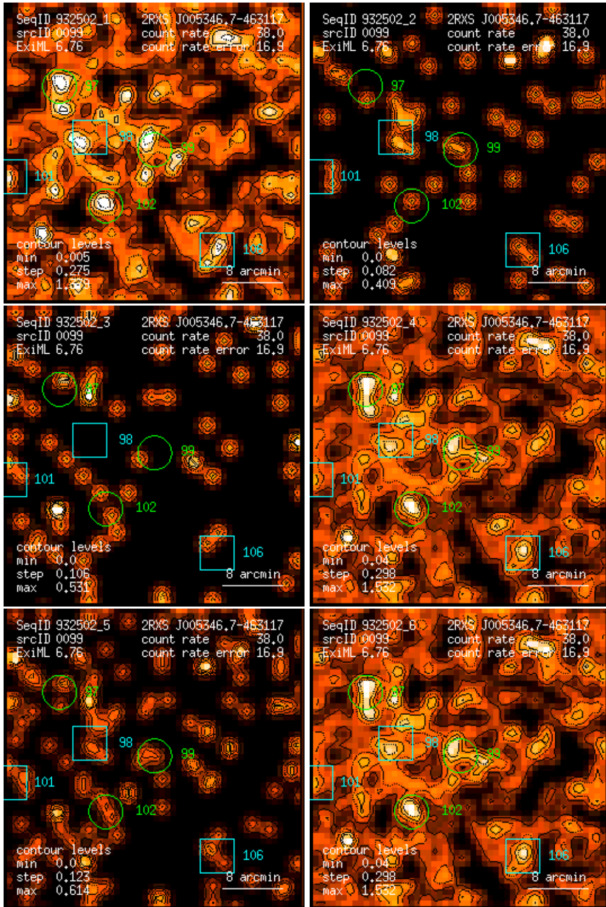
Figure 99: RASS 932502: detection 0099: band rate images, Gaussian filter: (1) PSPC channels 11 – 41, (2) 52 – 90, (3) 91 – 201, (4) 11 – 235, (5) 52 – 201, (6) 11 – 201. Broad band rates in counts/ks. Band rate contour levels in counts/ks/arcmin 2 .
