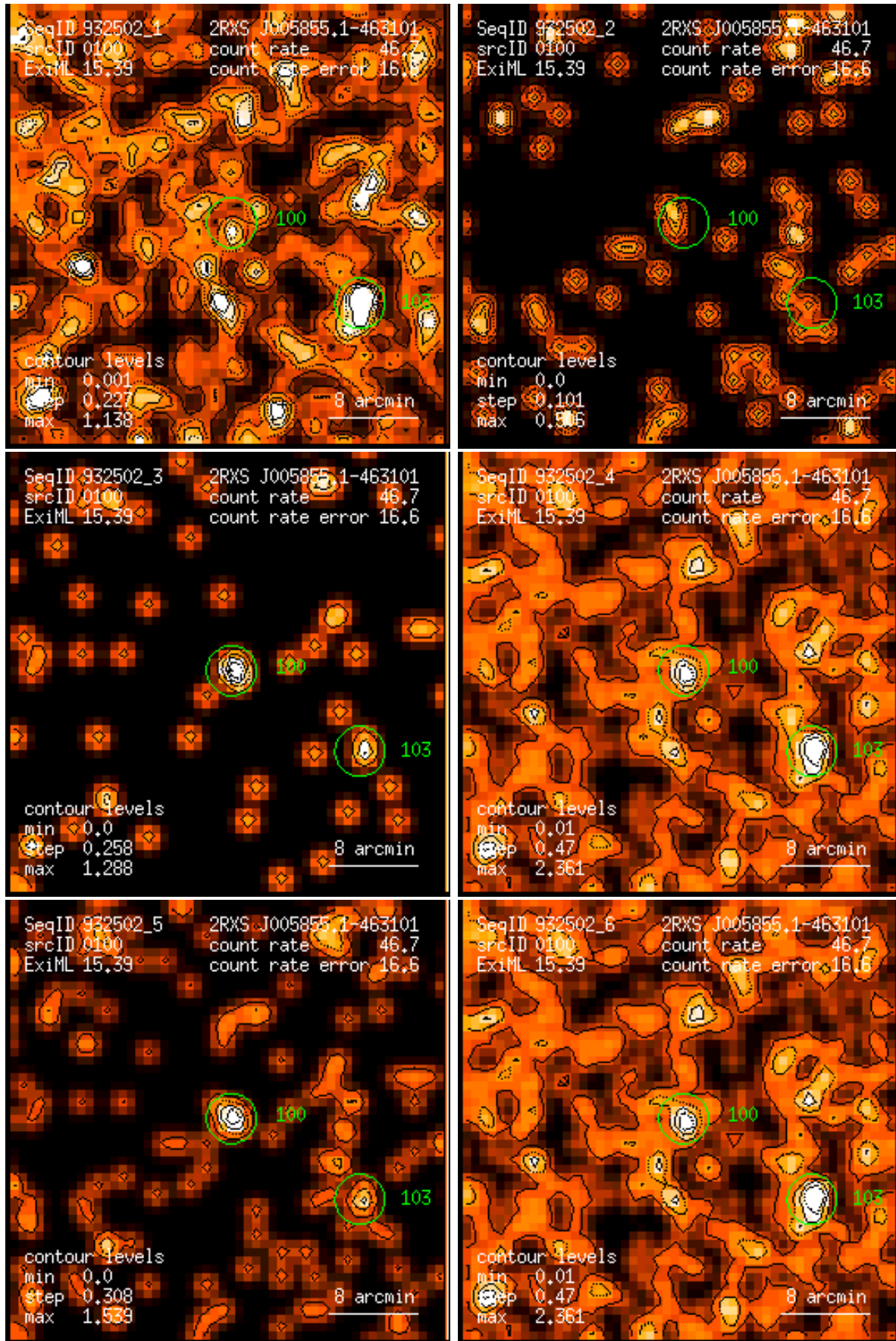
Figure 100: RASS 932502: detection 0100: band rate images, Gaussian filter: (1) PSPC channels 11 – 41, (2) 52 – 90, (3) 91 – 201, (4) 11 – 235, (5) 52 – 201, (6) 11 – 201. Broad band rates in counts/ks. Band rate contour levels in counts/ks/arcmin 2 .
