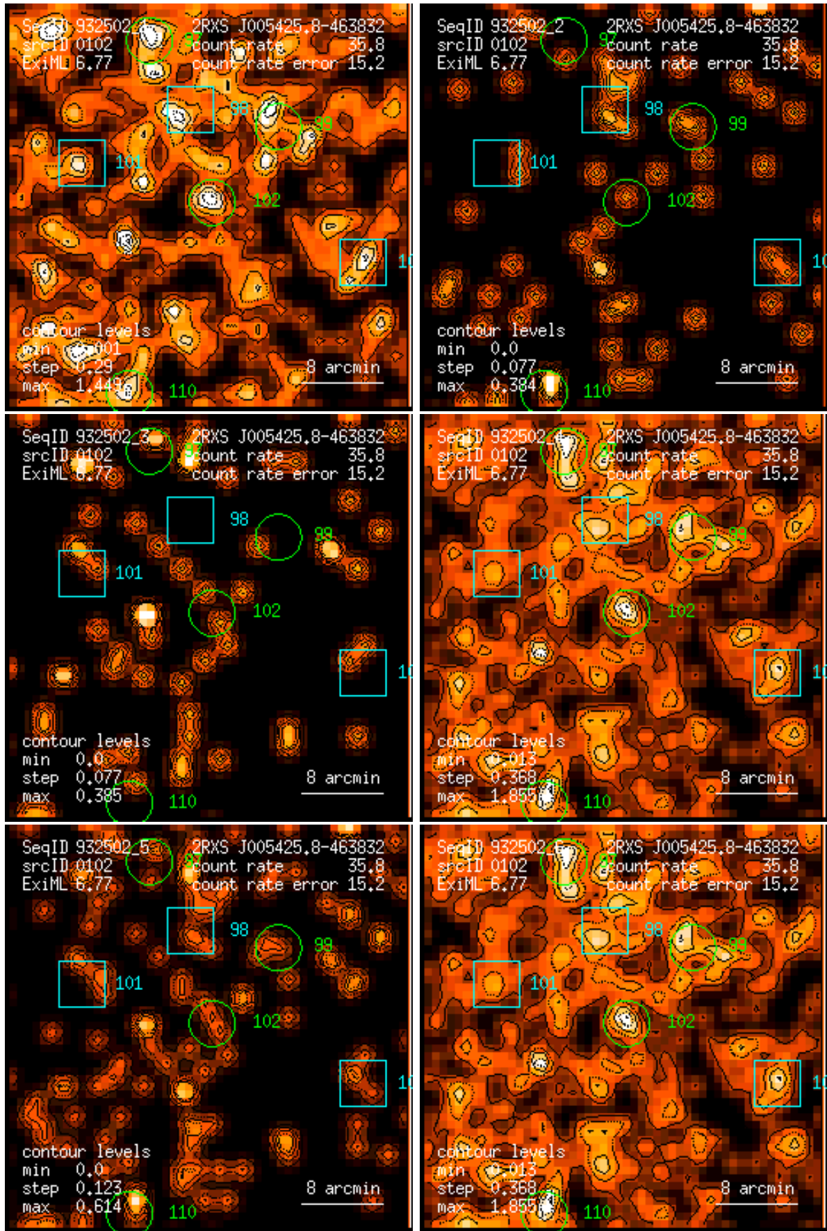
Figure 102: RASS 932502: detection 0102: band rate images, Gaussian filter: (1) PSPC channels 11 – 41, (2) 52 – 90, (3) 91 – 201, (4) 11 – 235, (5) 52 – 201, (6) 11 – 201. Broad band rates in counts/ks. Band rate contour levels in counts/ks/arcmin 2 .
