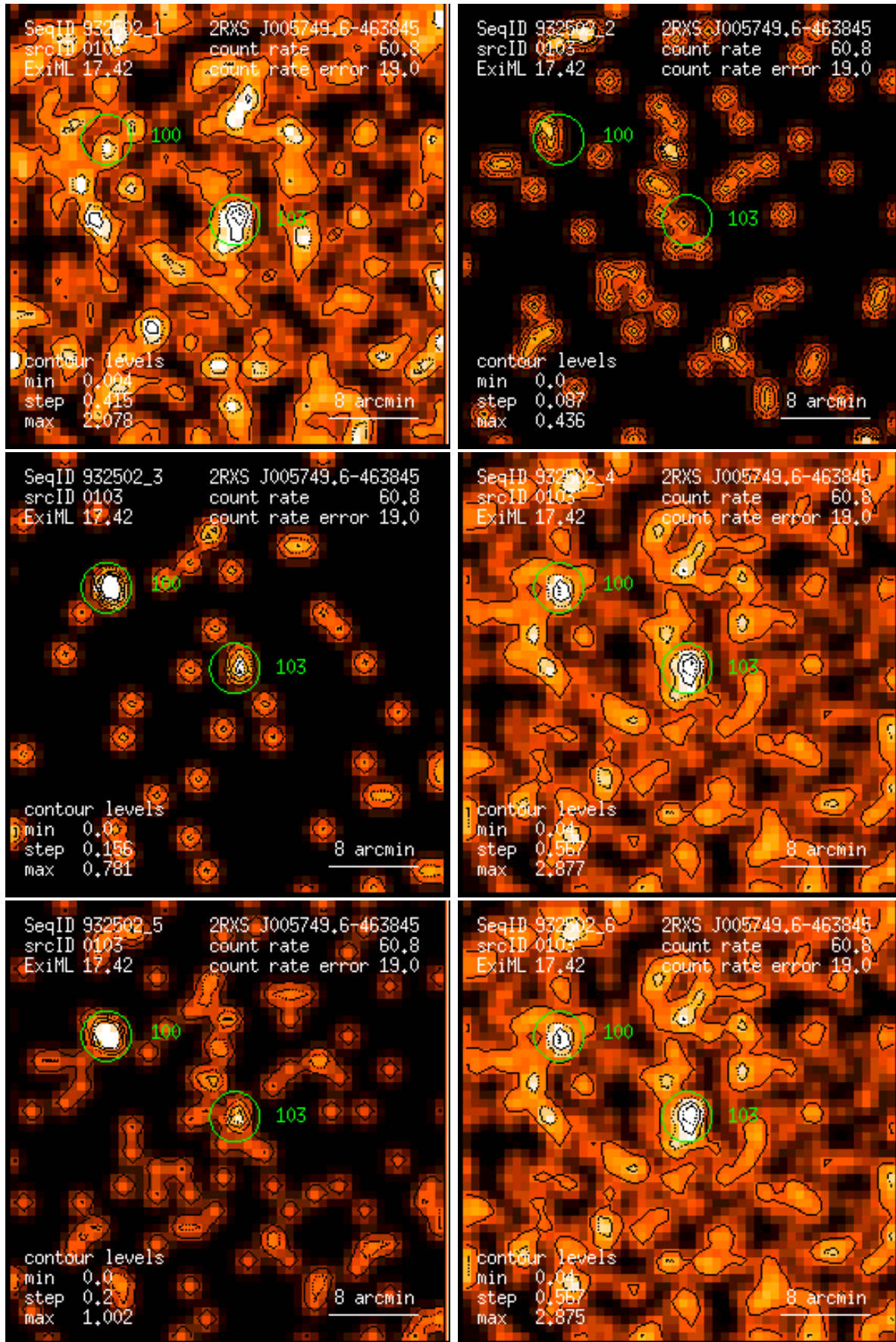
Figure 103: RASS 932502: detection 0103: band rate images, Gaussian filter: (1) PSPC channels 11 – 41, (2) 52 – 90, (3) 91 – 201, (4) 11 – 235, (5) 52 – 201, (6) 11 – 201. Broad band rates in counts/ks. Band rate contour levels in counts/ks/arcmin 2 .
