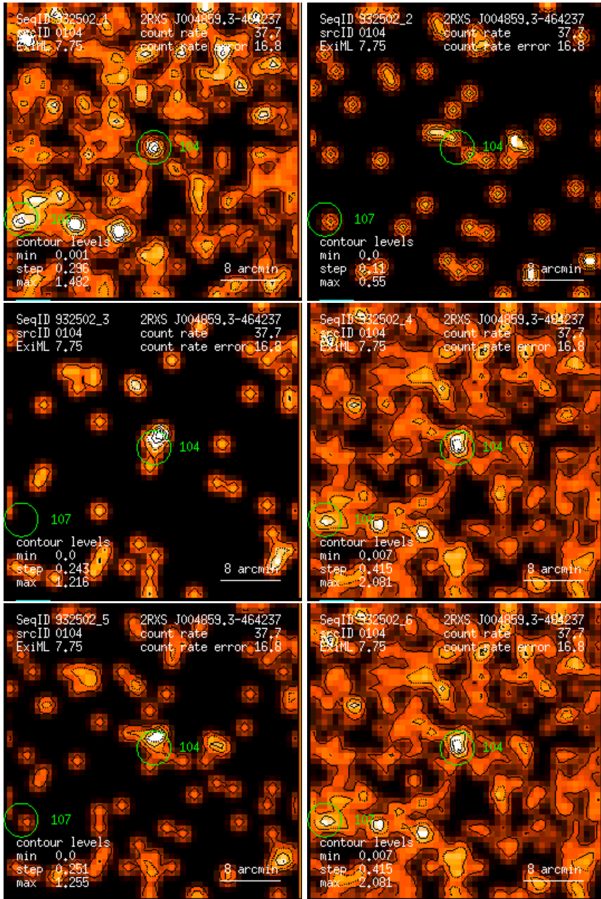
Figure 104: RASS 932502: detection 0104: band rate images, Gaussian filter: (1) PSPC channels 11 – 41, (2) 52 – 90, (3) 91 – 201, (4) 11 – 235, (5) 52 – 201, (6) 11 – 201. Broad band rates in counts/ks. Band rate contour levels in counts/ks/arcmin 2 .
