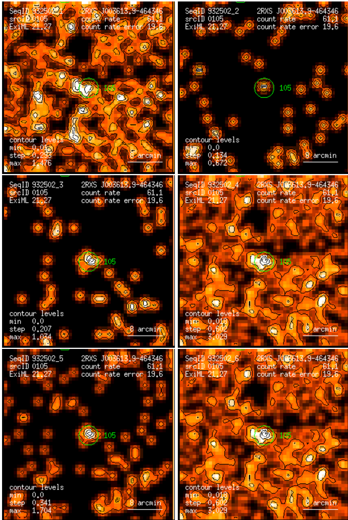
Figure 105: RASS 932502: detection 0105: band rate images, Gaussian filter: (1) PSPC channels 11 – 41, (2) 52 – 90, (3) 91 – 201, (4) 11 – 235, (5) 52 – 201, (6) 11 – 201. Broad band rates in counts/ks. Band rate contour levels in counts/ks/arcmin 2 .
