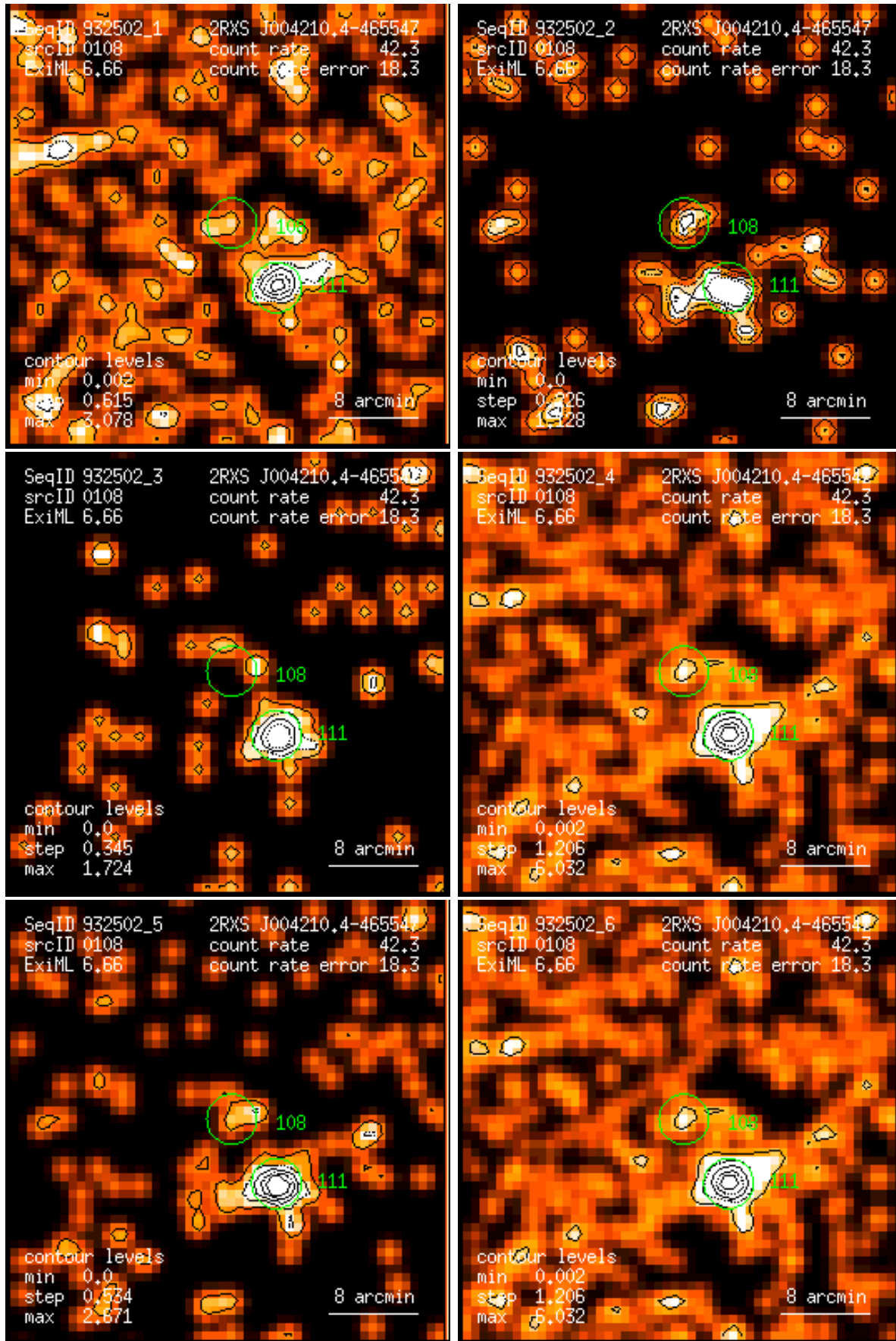
Figure 108: RASS 932502: detection 0108: band rate images, Gaussian filter: (1) PSPC channels 11 – 41, (2) 52 – 90, (3) 91 – 201, (4) 11 – 235, (5) 52 – 201, (6) 11 – 201. Broad band rates in counts/ks. Band rate contour levels in counts/ks/arcmin 2 .
