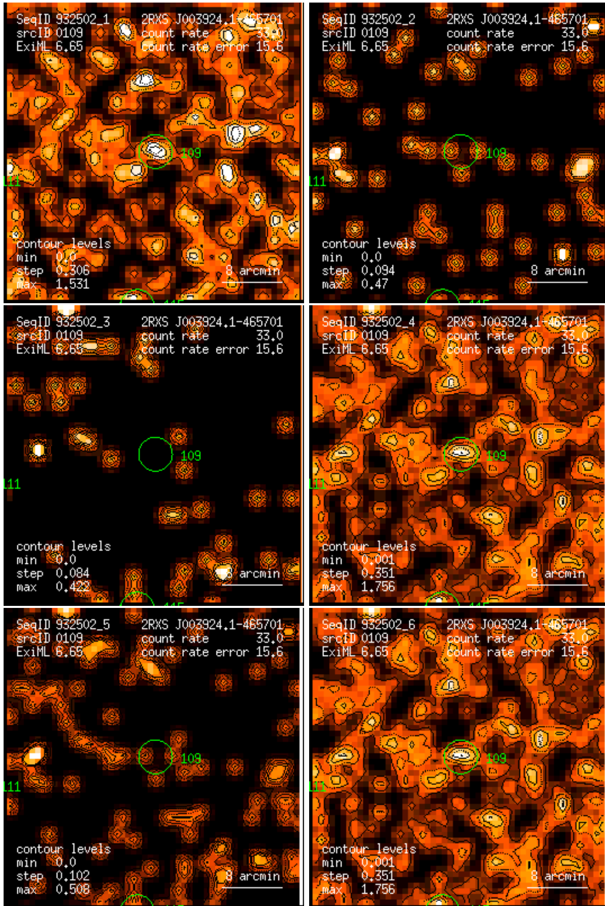
Figure 109: RASS 932502: detection 0109: band rate images, Gaussian filter: (1) PSPC channels 11 – 41, (2) 52 – 90, (3) 91 – 201, (4) 11 – 235, (5) 52 – 201, (6) 11 – 201. Broad band rates in counts/ks. Band rate contour levels in counts/ks/arcmin 2 .
