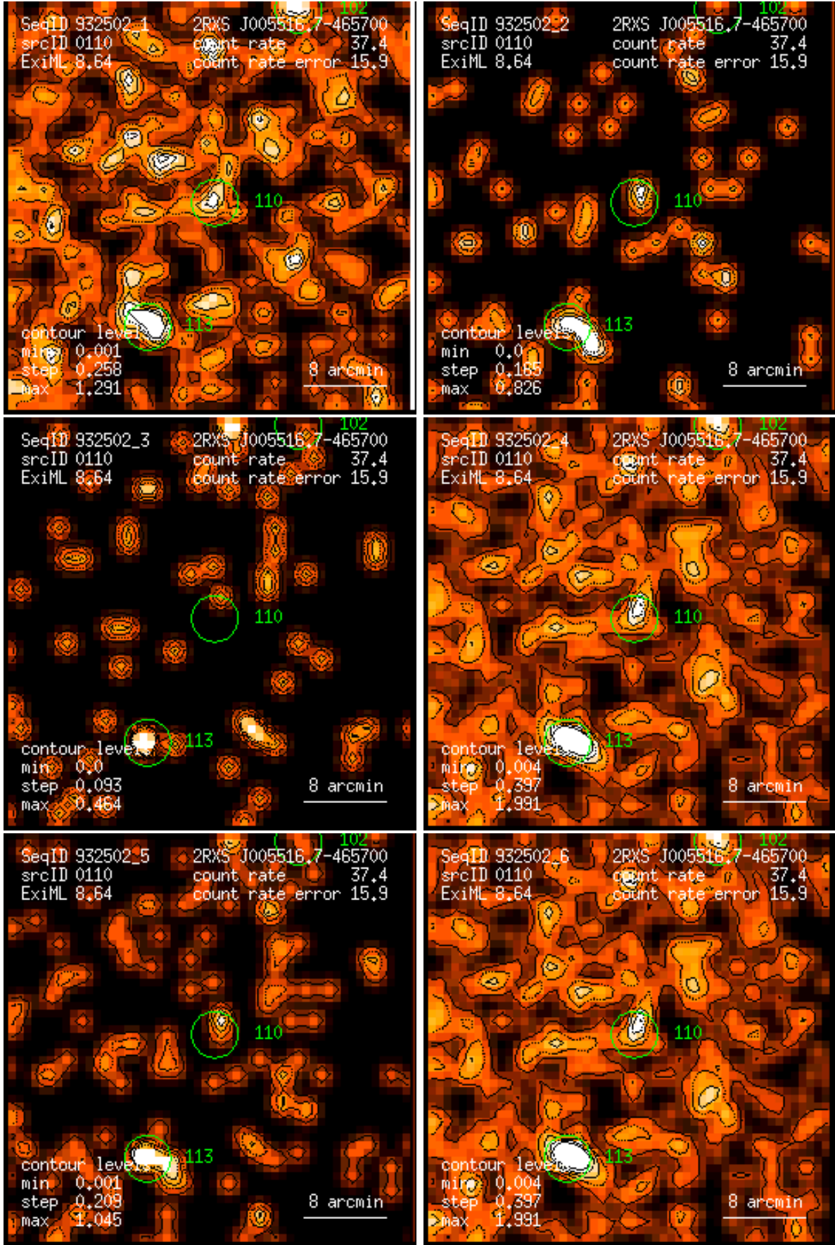
Figure 110: RASS 932502: detection 0110: band rate images, Gaussian filter: (1) PSPC channels 11 – 41, (2) 52 – 90, (3) 91 – 201, (4) 11 – 235, (5) 52 – 201, (6) 11 – 201. Broad band rates in counts/ks. Band rate contour levels in counts/ks/arcmin 2 .
