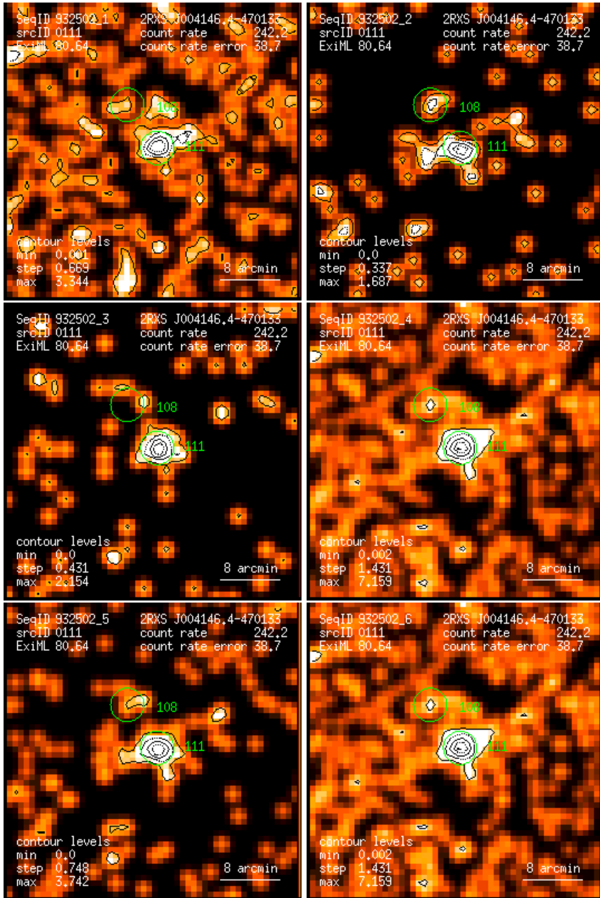
Figure 111: RASS 932502: detection 0111: band rate images, Gaussian filter: (1) PSPC channels 11 – 41, (2) 52 – 90, (3) 91 – 201, (4) 11 – 235, (5) 52 – 201, (6) 11 – 201. Broad band rates in counts/ks. Band rate contour levels in counts/ks/arcmin 2 .
