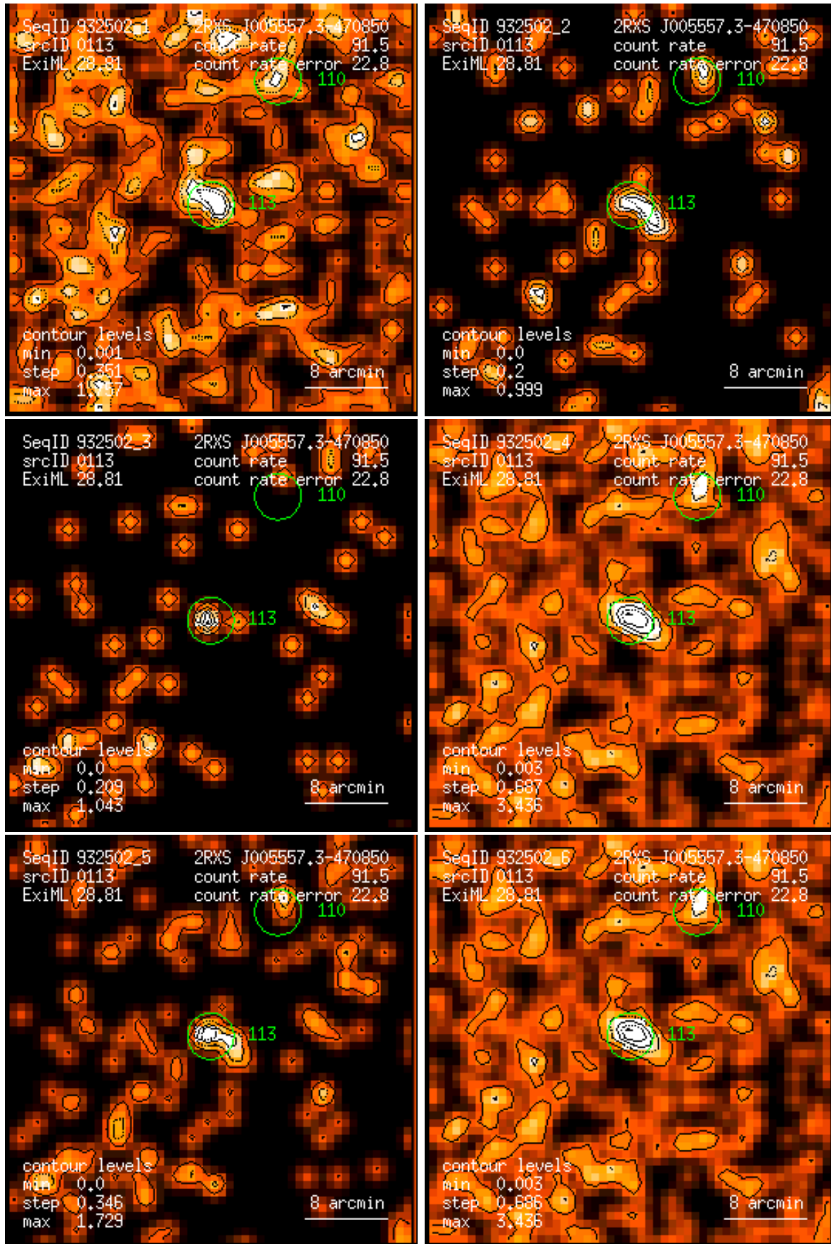
Figure 113: RASS 932502: detection 0113: band rate images, Gaussian filter: (1) PSPC channels 11 – 41, (2) 52 – 90, (3) 91 – 201, (4) 11 – 235, (5) 52 – 201, (6) 11 – 201. Broad band rates in counts/ks. Band rate contour levels in counts/ks/arcmin 2 .
