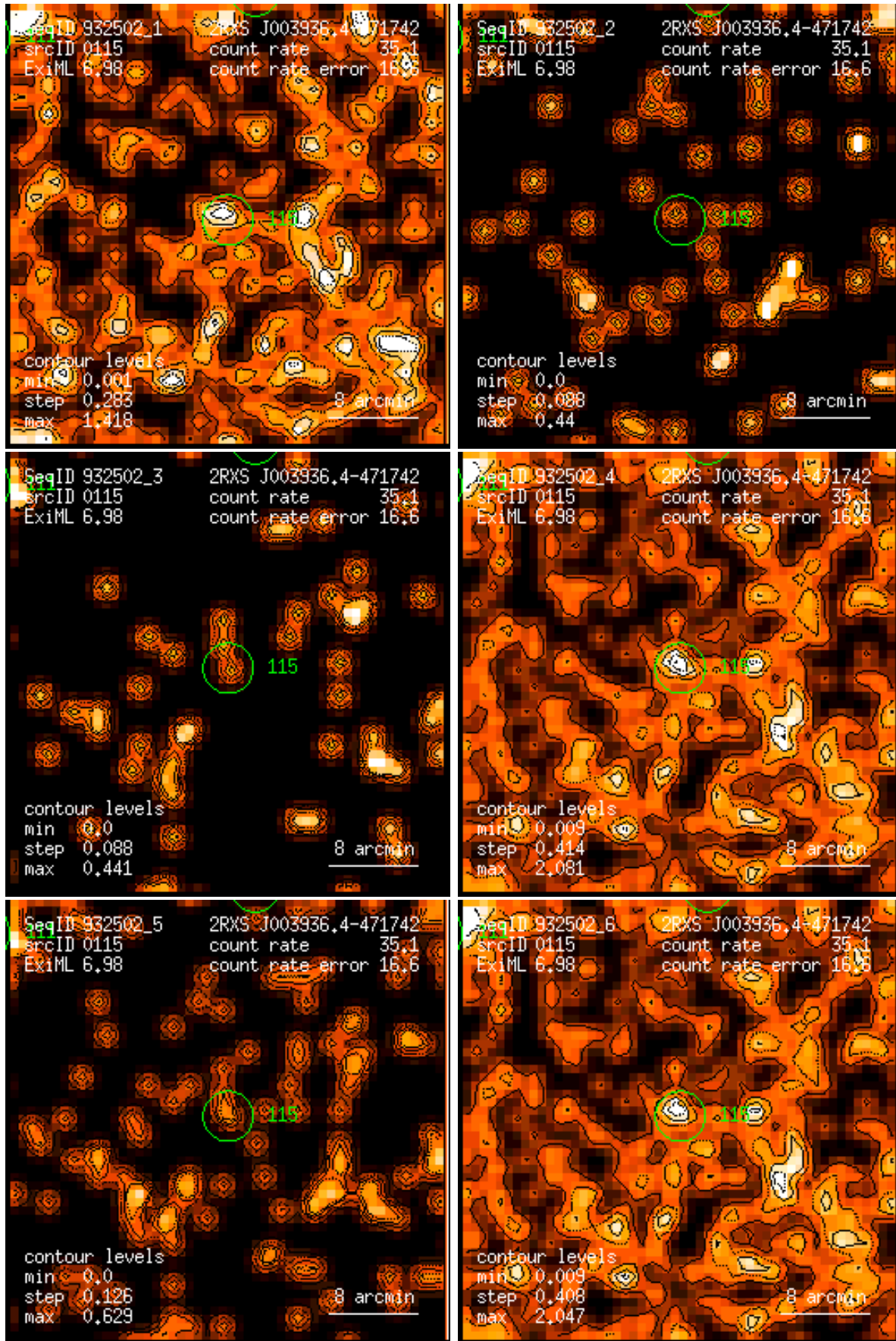
Figure 115: RASS 932502: detection 0115: band rate images, Gaussian filter: (1) PSPC channels 11 – 41, (2) 52 – 90, (3) 91 – 201, (4) 11 – 235, (5) 52 – 201, (6) 11 – 201. Broad band rates in counts/ks. Band rate contour levels in counts/ks/arcmin 2 .
