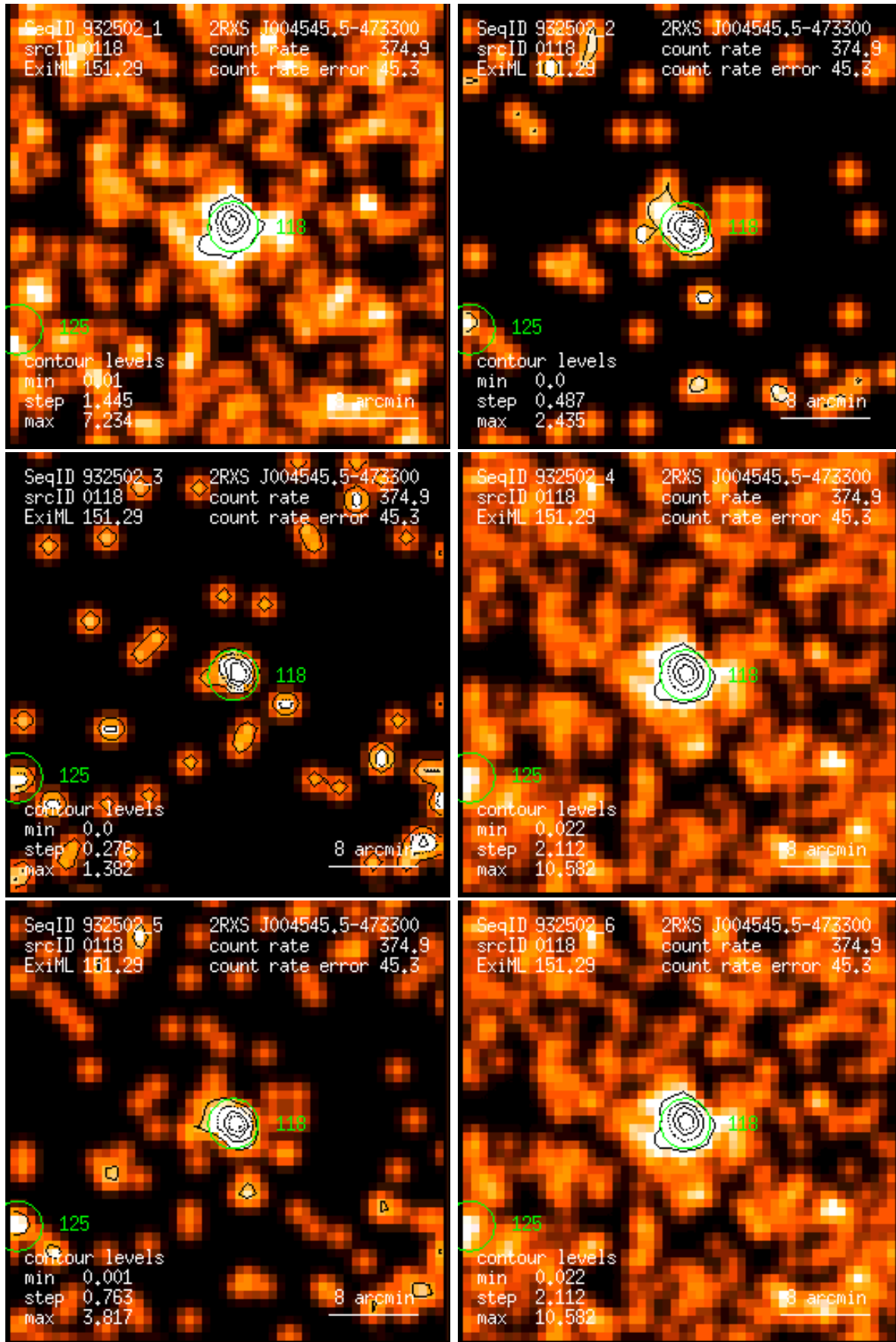
Figure 118: RASS 932502: detection 0118: band rate images, Gaussian filter: (1) PSPC channels 11 – 41, (2) 52 – 90, (3) 91 – 201, (4) 11 – 235, (5) 52 – 201, (6) 11 – 201. Broad band rates in counts/ks. Band rate contour levels in counts/ks/arcmin 2 .
