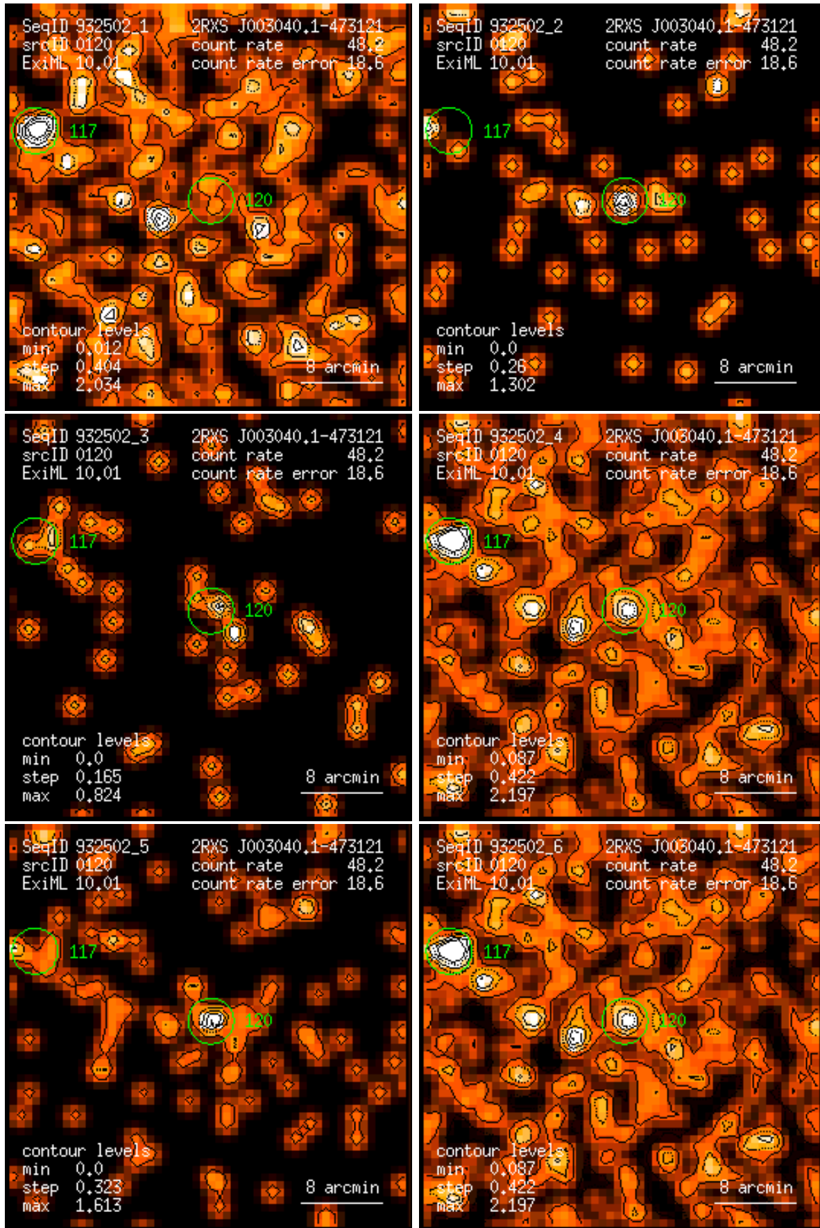
Figure 120: RASS 932502: detection 0120: band rate images, Gaussian filter: (1) PSPC channels 11 – 41, (2) 52 – 90, (3) 91 – 201, (4) 11 – 235, (5) 52 – 201, (6) 11 – 201. Broad band rates in counts/ks. Band rate contour levels in counts/ks/arcmin 2 .
