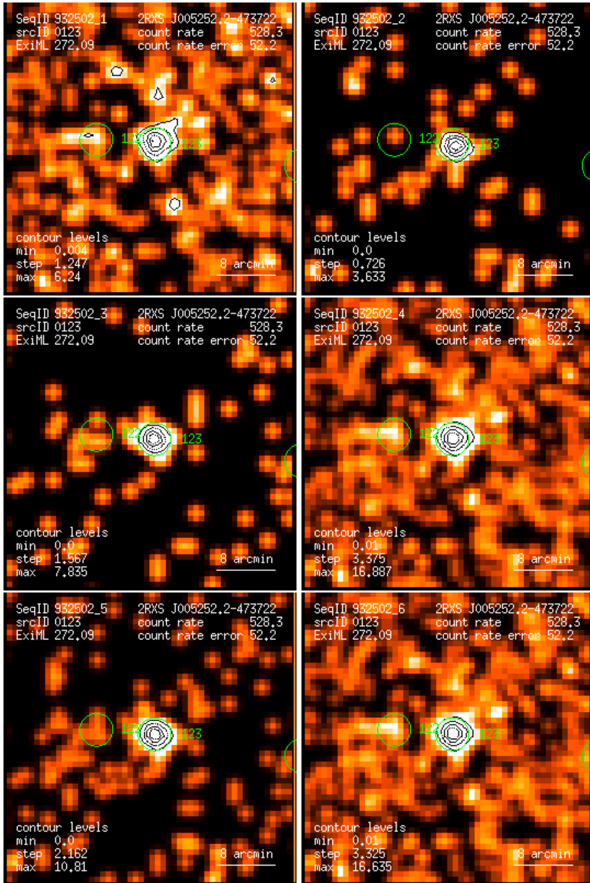
Figure 123: RASS 932502: detection 0123: band rate images, Gaussian filter: (1) PSPC channels 11 – 41, (2) 52 – 90, (3) 91 – 201, (4) 11 – 235, (5) 52 – 201, (6) 11 – 201. Broad band rates in counts/ks. Band rate contour levels in counts/ks/arcmin 2 .
