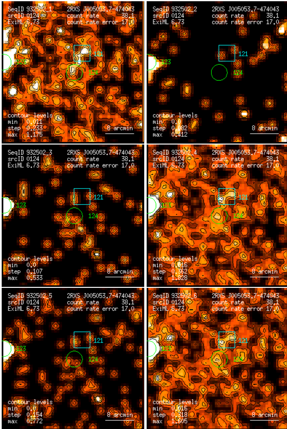
Figure 124: RASS 932502: detection 0124: band rate images, Gaussian filter: (1) PSPC channels 11 – 41, (2) 52 – 90, (3) 91 – 201, (4) 11 – 235, (5) 52 – 201, (6) 11 – 201. Broad band rates in counts/ks. Band rate contour levels in counts/ks/arcmin 2 .
