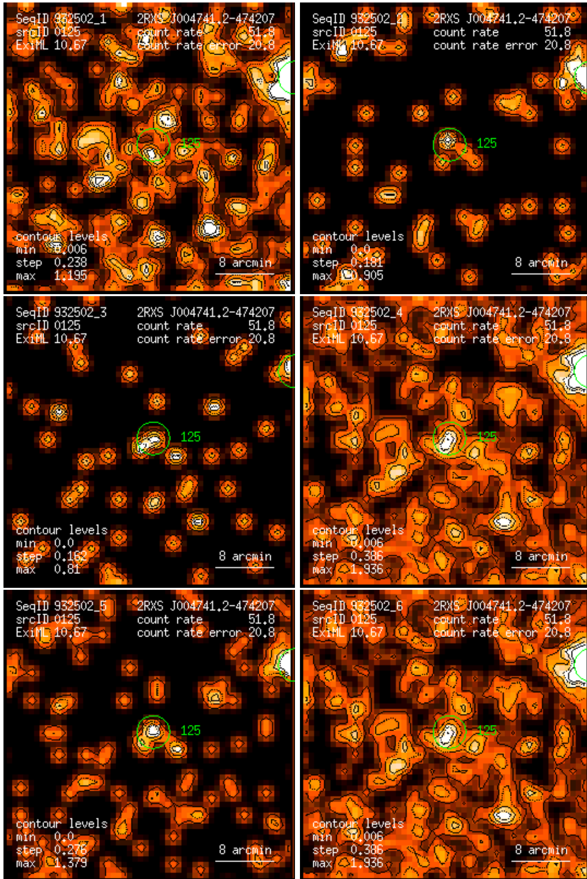
Figure 125: RASS 932502: detection 0125: band rate images, Gaussian filter: (1) PSPC channels 11 – 41, (2) 52 – 90, (3) 91 – 201, (4) 11 – 235, (5) 52 – 201, (6) 11 – 201. Broad band rates in counts/ks. Band rate contour levels in counts/ks/arcmin 2 .
