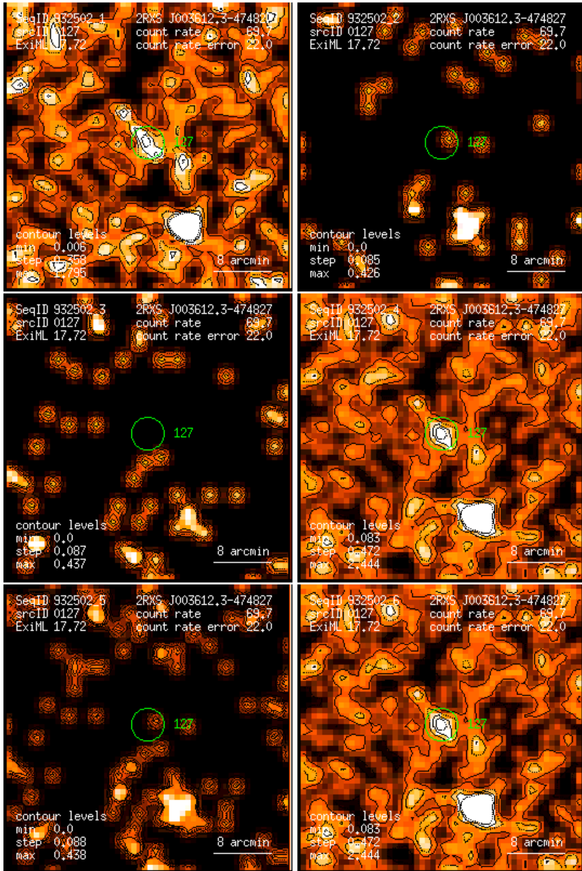
Figure 127: RASS 932502: detection 0127: band rate images, Gaussian filter: (1) PSPC channels 11 – 41, (2) 52 – 90, (3) 91 – 201, (4) 11 – 235, (5) 52 – 201, (6) 11 – 201. Broad band rates in counts/ks. Band rate contour levels in counts/ks/arcmin 2 .
