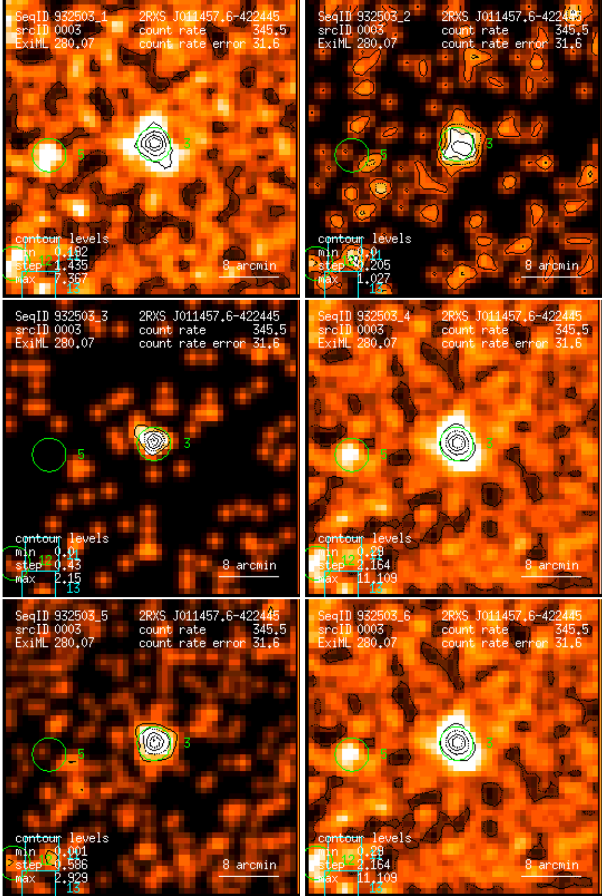
Figure 3: RASS 932503: detection 0003: band rate images, Gaussian filter: (1) PSPC channels 11 – 41, (2) 52 – 90, (3) 91 – 201, (4) 11 – 235, (5) 52 – 201, (6) 11 – 201. Broad band rates in counts/ks. Band rate contour levels in counts/ks/arcmin 2 .
