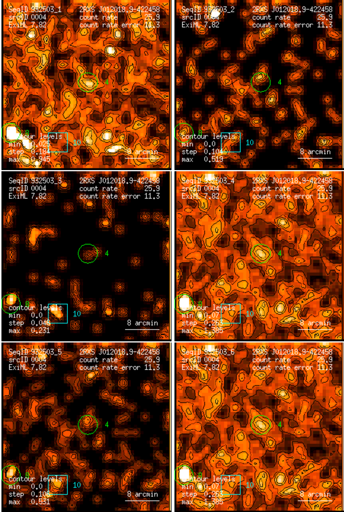
Figure 4: RASS 932503: detection 0004: band rate images, Gaussian filter: (1) PSPC channels 11 – 41, (2) 52 – 90, (3) 91 – 201, (4) 11 – 235, (5) 52 – 201, (6) 11 – 201. Broad band rates in counts/ks. Band rate contour levels in counts/ks/arcmin 2 .
