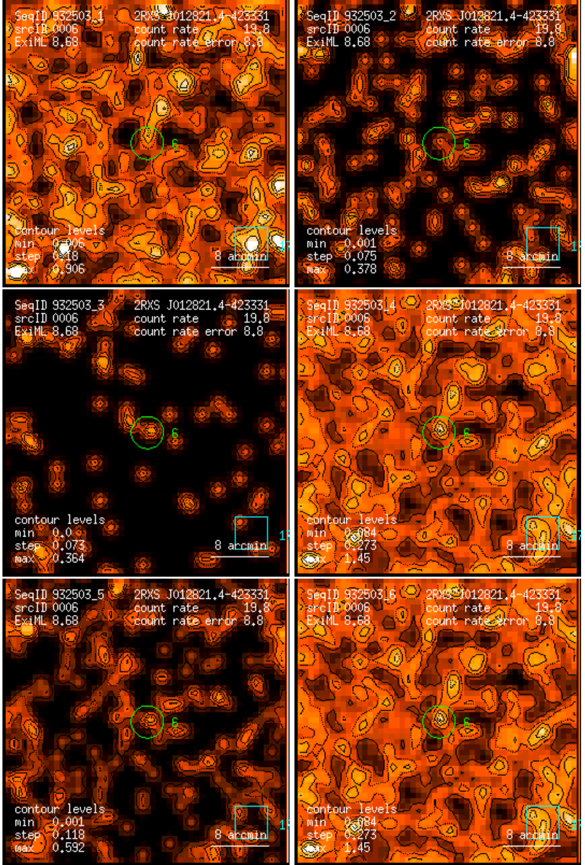
Figure 6: RASS 932503: detection 0006: band rate images, Gaussian filter: (1) PSPC channels 11 – 41, (2) 52 – 90, (3) 91 – 201, (4) 11 – 235, (5) 52 – 201, (6) 11 – 201. Broad band rates in counts/ks. Band rate contour levels in counts/ks/arcmin 2 .
