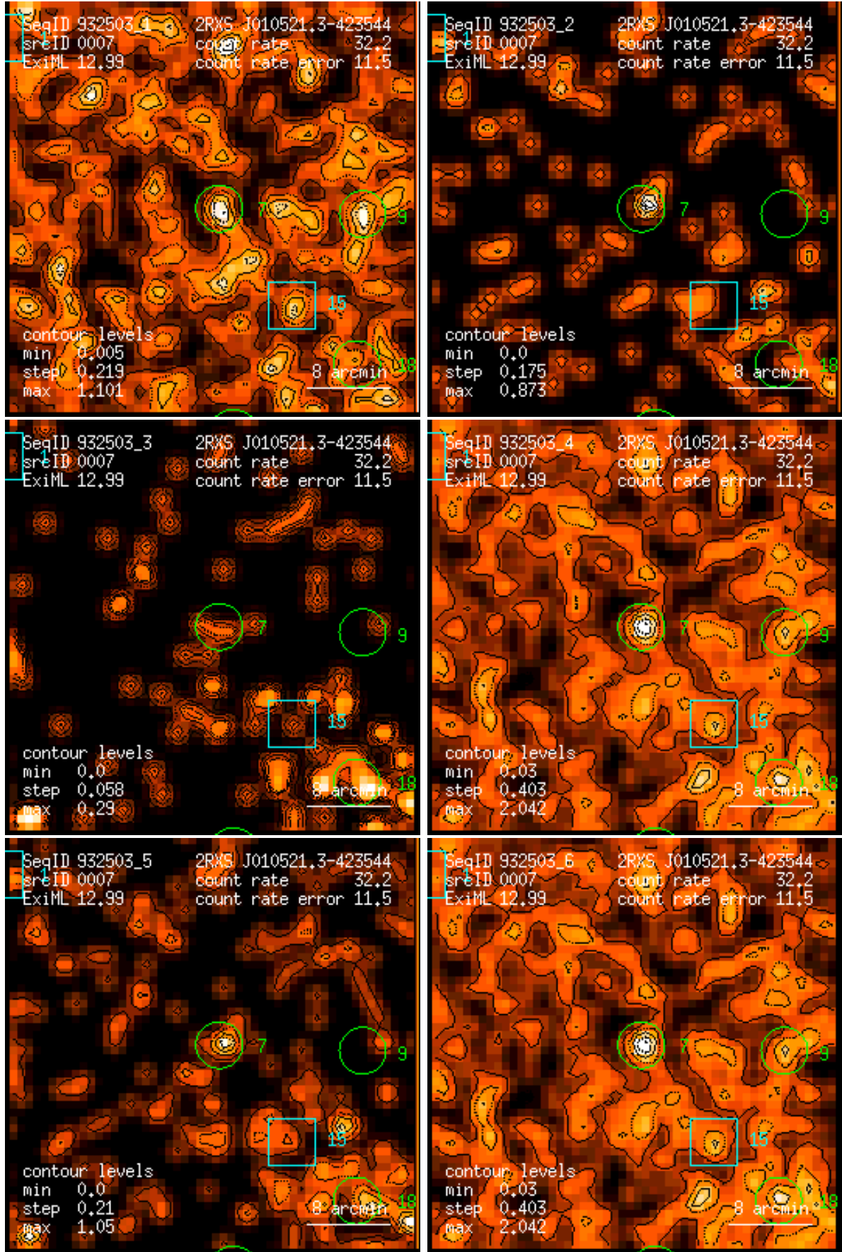
Figure 7: RASS 932503: detection 0007: band rate images, Gaussian filter: (1) PSPC channels 11 – 41, (2) 52 – 90, (3) 91 – 201, (4) 11 – 235, (5) 52 – 201, (6) 11 – 201. Broad band rates in counts/ks. Band rate contour levels in counts/ks/arcmin 2 .
