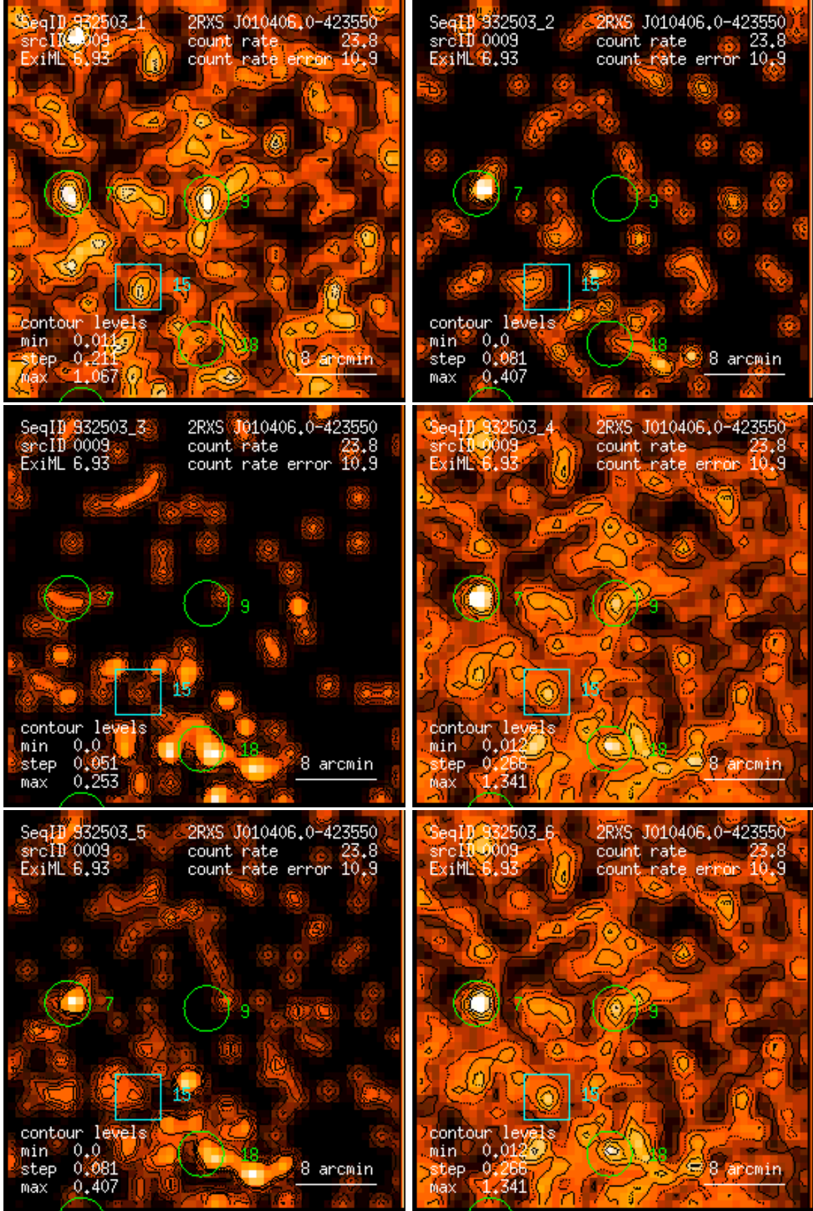
Figure 9: RASS 932503: detection 0009: band rate images, Gaussian filter: (1) PSPC channels 11 – 41, (2) 52 – 90, (3) 91 – 201, (4) 11 – 235, (5) 52 – 201, (6) 11 – 201. Broad band rates in counts/ks. Band rate contour levels in counts/ks/arcmin 2 .
