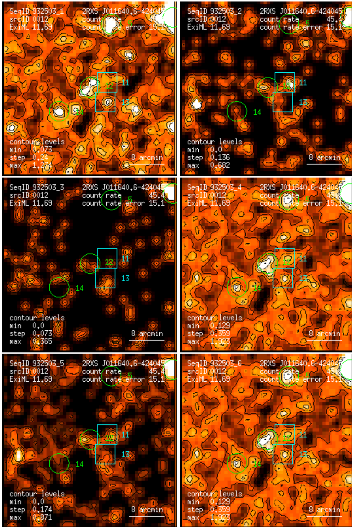
Figure 12: RASS 932503: detection 0012: band rate images, Gaussian filter: (1) PSPC channels 11 – 41, (2) 52 – 90, (3) 91 – 201, (4) 11 – 235, (5) 52 – 201, (6) 11 – 201. Broad band rates in counts/ks. Band rate contour levels in counts/ks/arcmin 2 .
