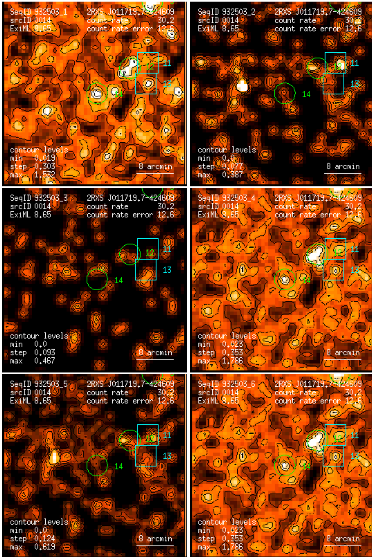
Figure 14: RASS 932503: detection 0014: band rate images, Gaussian filter: (1) PSPC channels 11 – 41, (2) 52 – 90, (3) 91 – 201, (4) 11 – 235, (5) 52 – 201, (6) 11 – 201. Broad band rates in counts/ks. Band rate contour levels in counts/ks/arcmin 2 .
