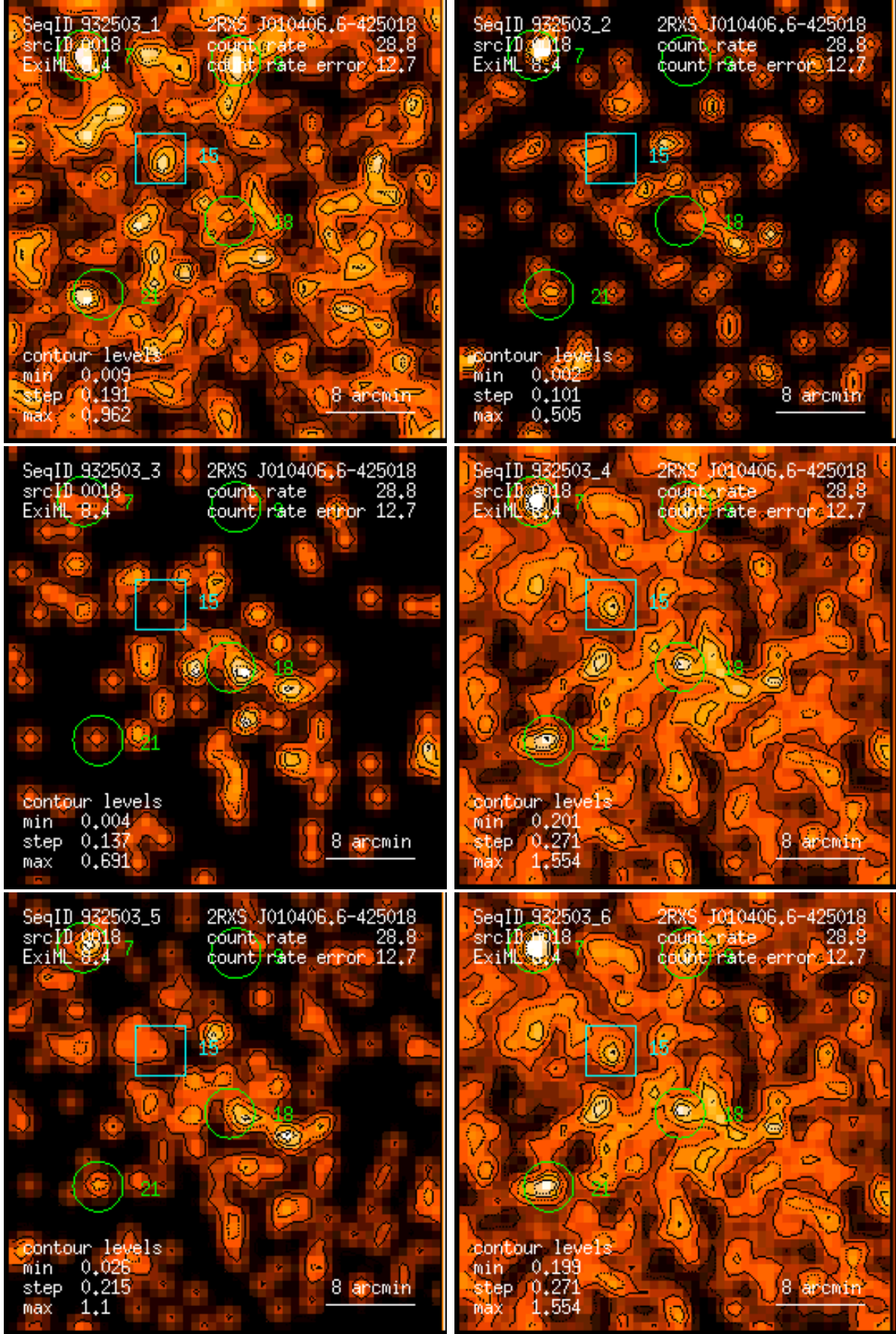
Figure 18: RASS 932503: detection 0018: band rate images, Gaussian filter: (1) PSPC channels 11 – 41, (2) 52 – 90, (3) 91 – 201, (4) 11 – 235, (5) 52 – 201, (6) 11 – 201. Broad band rates in counts/ks. Band rate contour levels in counts/ks/arcmin 2 .
