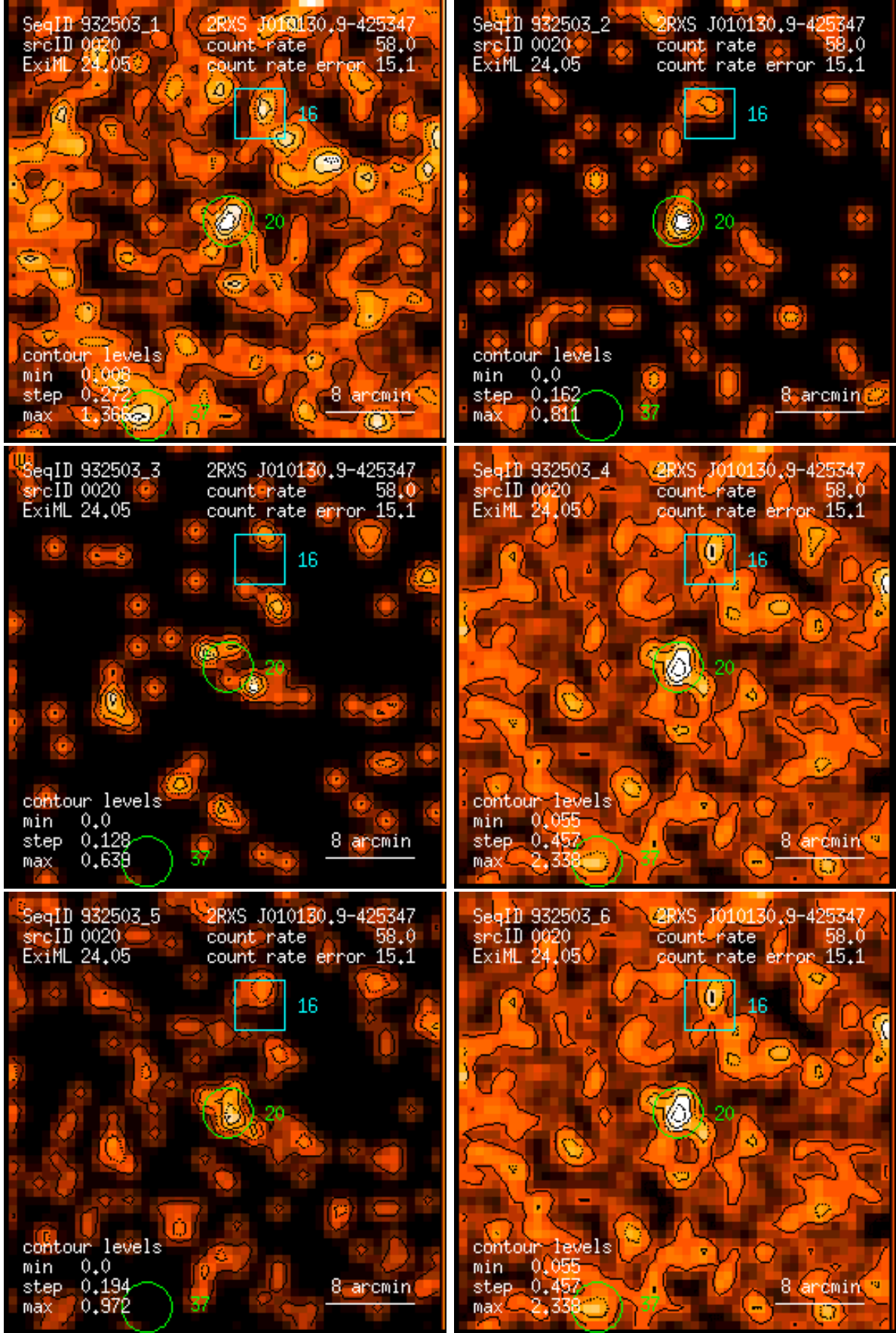
Figure 20: RASS 932503: detection 0020: band rate images, Gaussian filter: (1) PSPC channels 11 – 41, (2) 52 – 90, (3) 91 – 201, (4) 11 – 235, (5) 52 – 201, (6) 11 – 201. Broad band rates in counts/ks. Band rate contour levels in counts/ks/arcmin 2 .
