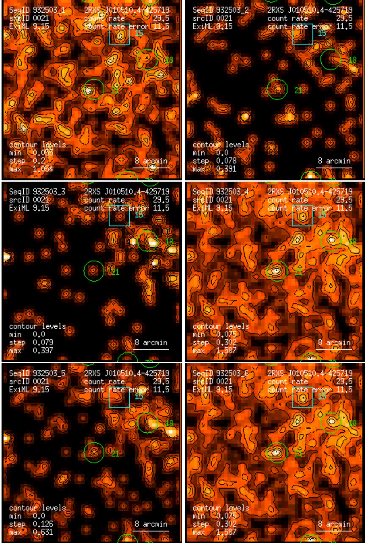
Figure 21: RASS 932503: detection 0021: band rate images, Gaussian filter: (1) PSPC channels 11 – 41, (2) 52 – 90, (3) 91 – 201, (4) 11 – 235, (5) 52 – 201, (6) 11 – 201. Broad band rates in counts/ks. Band rate contour levels in counts/ks/arcmin 2 .
