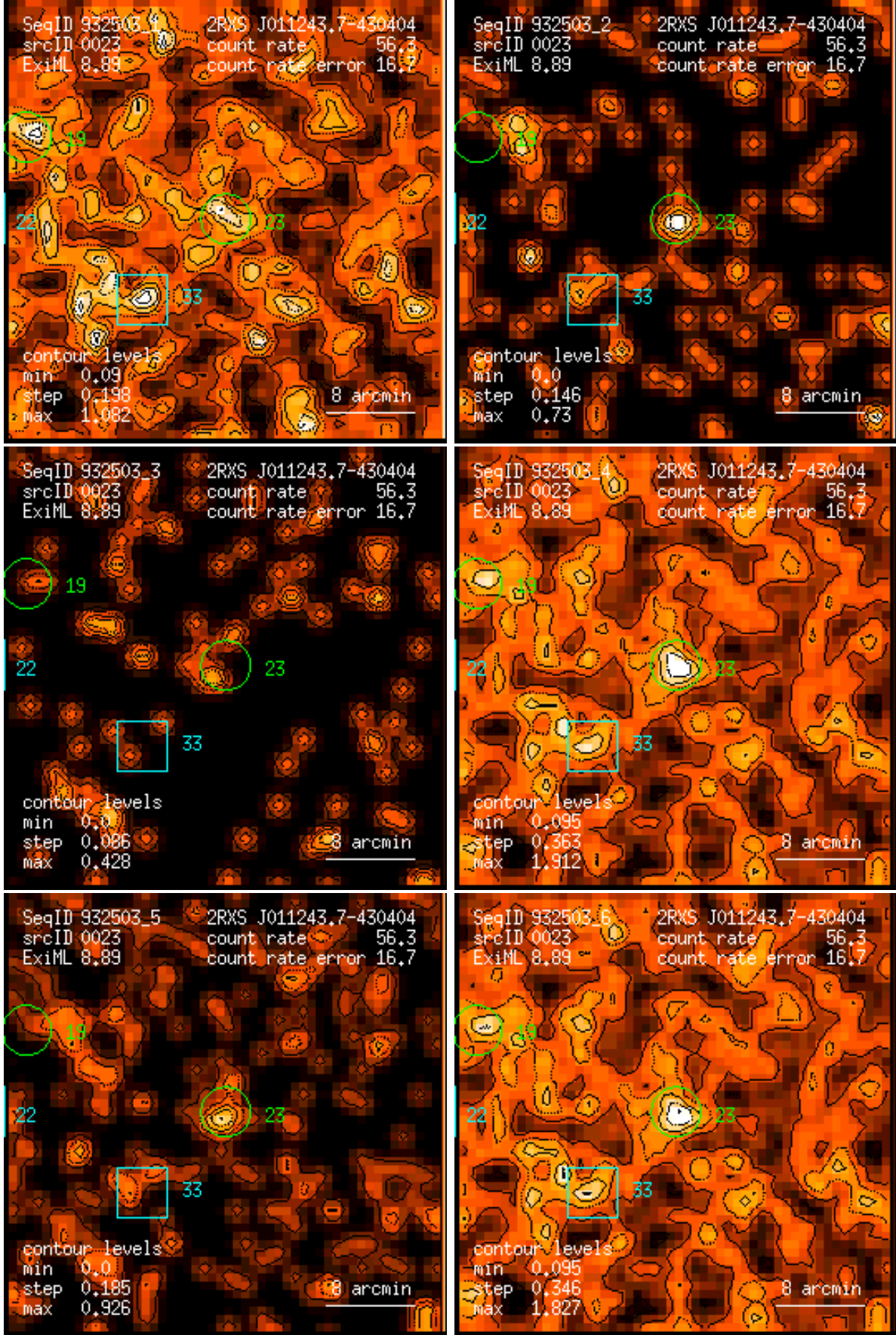
Figure 23: RASS 932503: detection 0023: band rate images, Gaussian filter: (1) PSPC channels 11 – 41, (2) 52 – 90, (3) 91 – 201, (4) 11 – 235, (5) 52 – 201, (6) 11 – 201. Broad band rates in counts/ks. Band rate contour levels in counts/ks/arcmin 2 .
