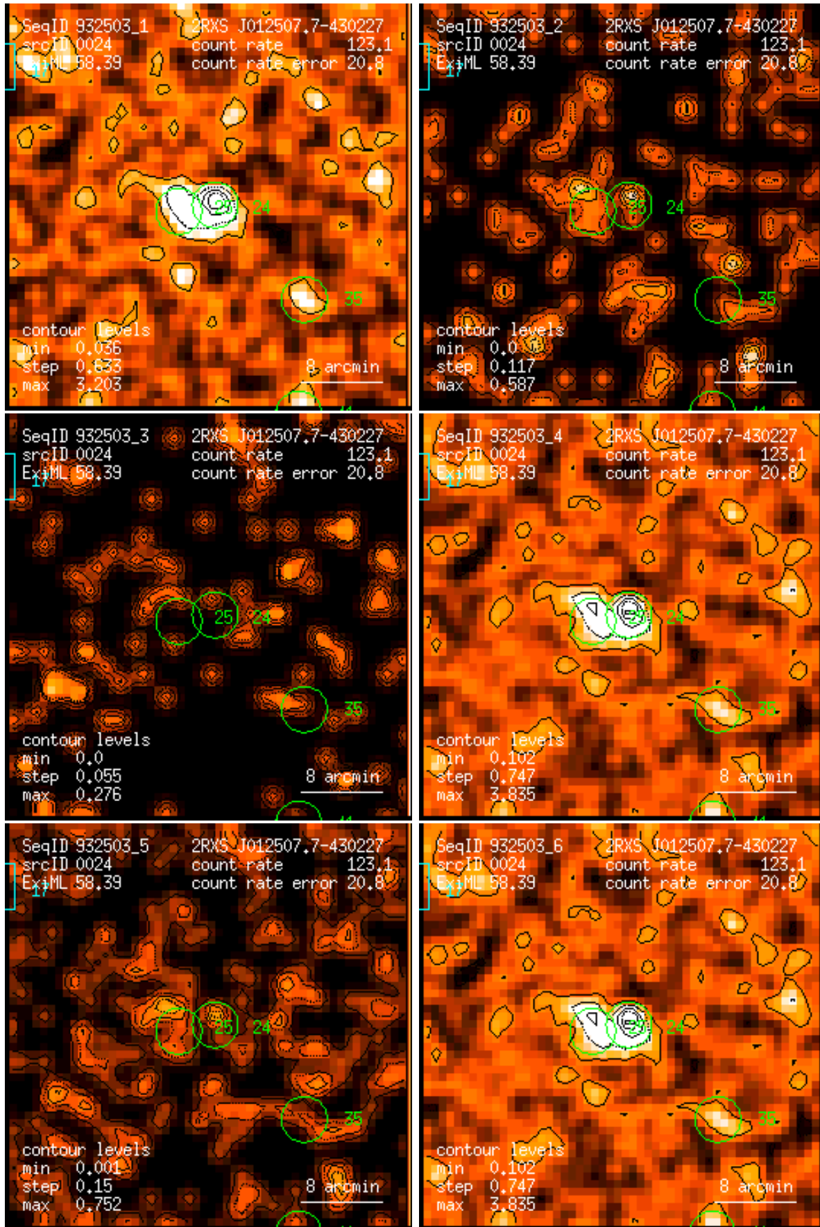
Figure 24: RASS 932503: detection 0024: band rate images, Gaussian filter: (1) PSPC channels 11 – 41, (2) 52 – 90, (3) 91 – 201, (4) 11 – 235, (5) 52 – 201, (6) 11 – 201. Broad band rates in counts/ks. Band rate contour levels in counts/ks/arcmin 2 .
