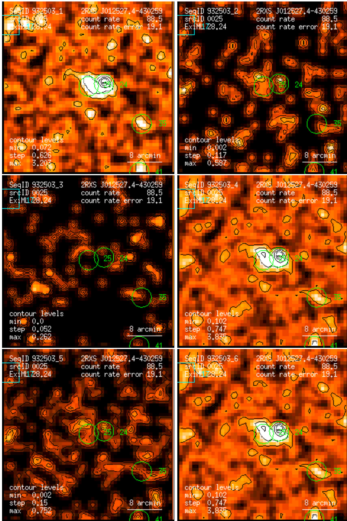
Figure 25: RASS 932503: detection 0025: band rate images, Gaussian filter: (1) PSPC channels 11 – 41, (2) 52 – 90, (3) 91 – 201, (4) 11 – 235, (5) 52 – 201, (6) 11 – 201. Broad band rates in counts/ks. Band rate contour levels in counts/ks/arcmin 2 .
