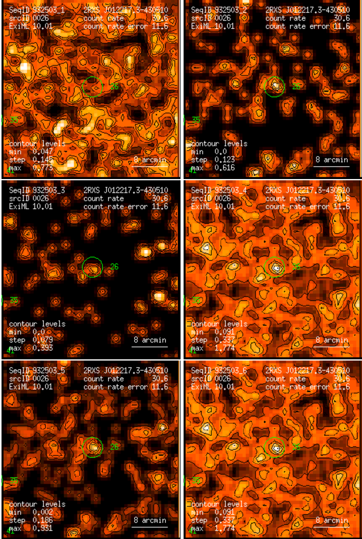
Figure 26: RASS 932503: detection 0026: band rate images, Gaussian filter: (1) PSPC channels 11 – 41, (2) 52 – 90, (3) 91 – 201, (4) 11 – 235, (5) 52 – 201, (6) 11 – 201. Broad band rates in counts/ks. Band rate contour levels in counts/ks/arcmin 2 .
