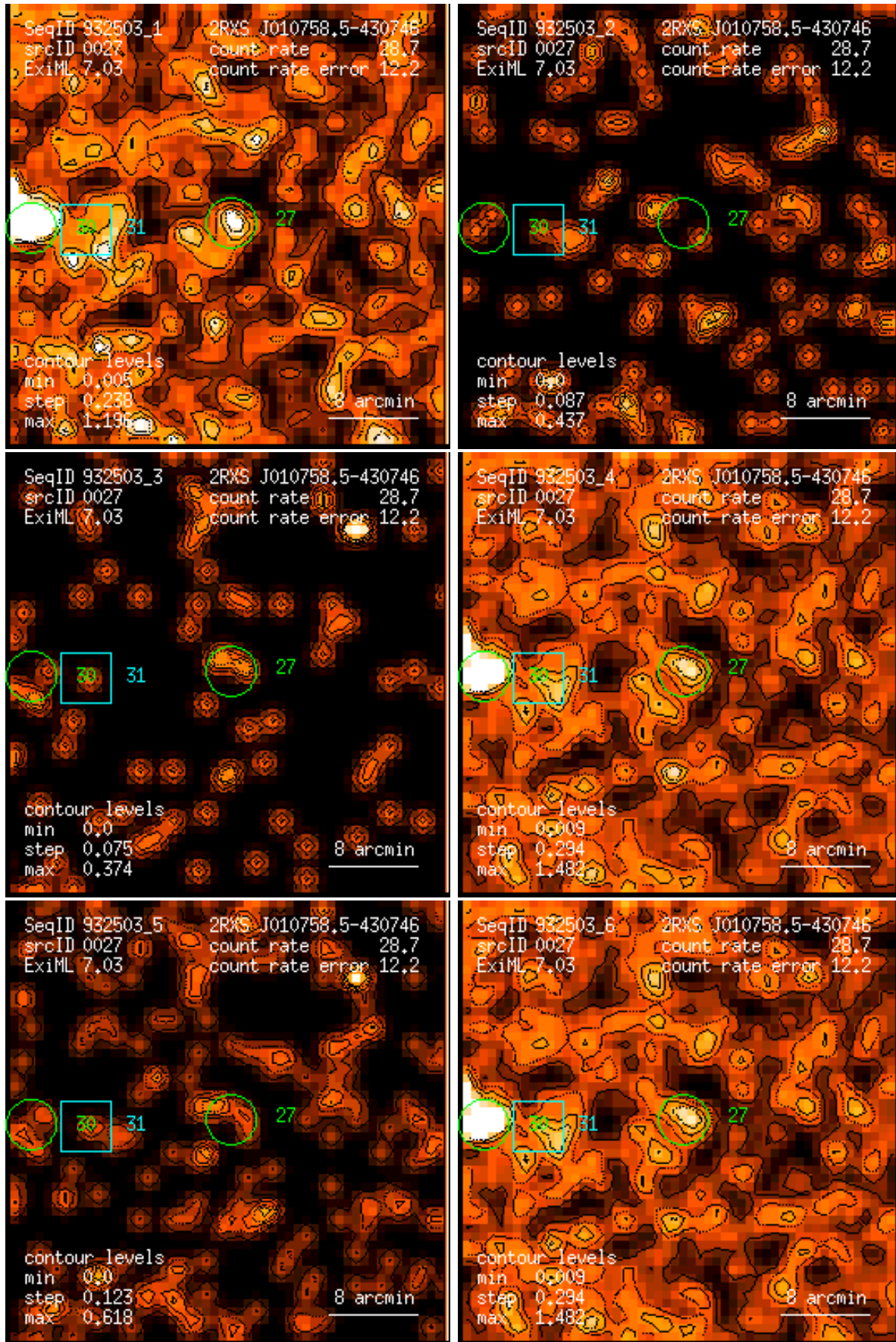
Figure 27: RASS 932503: detection 0027: band rate images, Gaussian filter: (1) PSPC channels 11 – 41, (2) 52 – 90, (3) 91 – 201, (4) 11 – 235, (5) 52 – 201, (6) 11 – 201. Broad band rates in counts/ks. Band rate contour levels in counts/ks/arcmin 2 .
