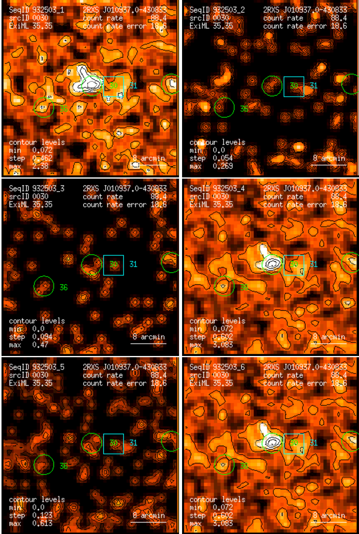
Figure 30: RASS 932503: detection 0030: band rate images, Gaussian filter: (1) PSPC channels 11 – 41, (2) 52 – 90, (3) 91 – 201, (4) 11 – 235, (5) 52 – 201, (6) 11 – 201. Broad band rates in counts/ks. Band rate contour levels in counts/ks/arcmin 2 .
