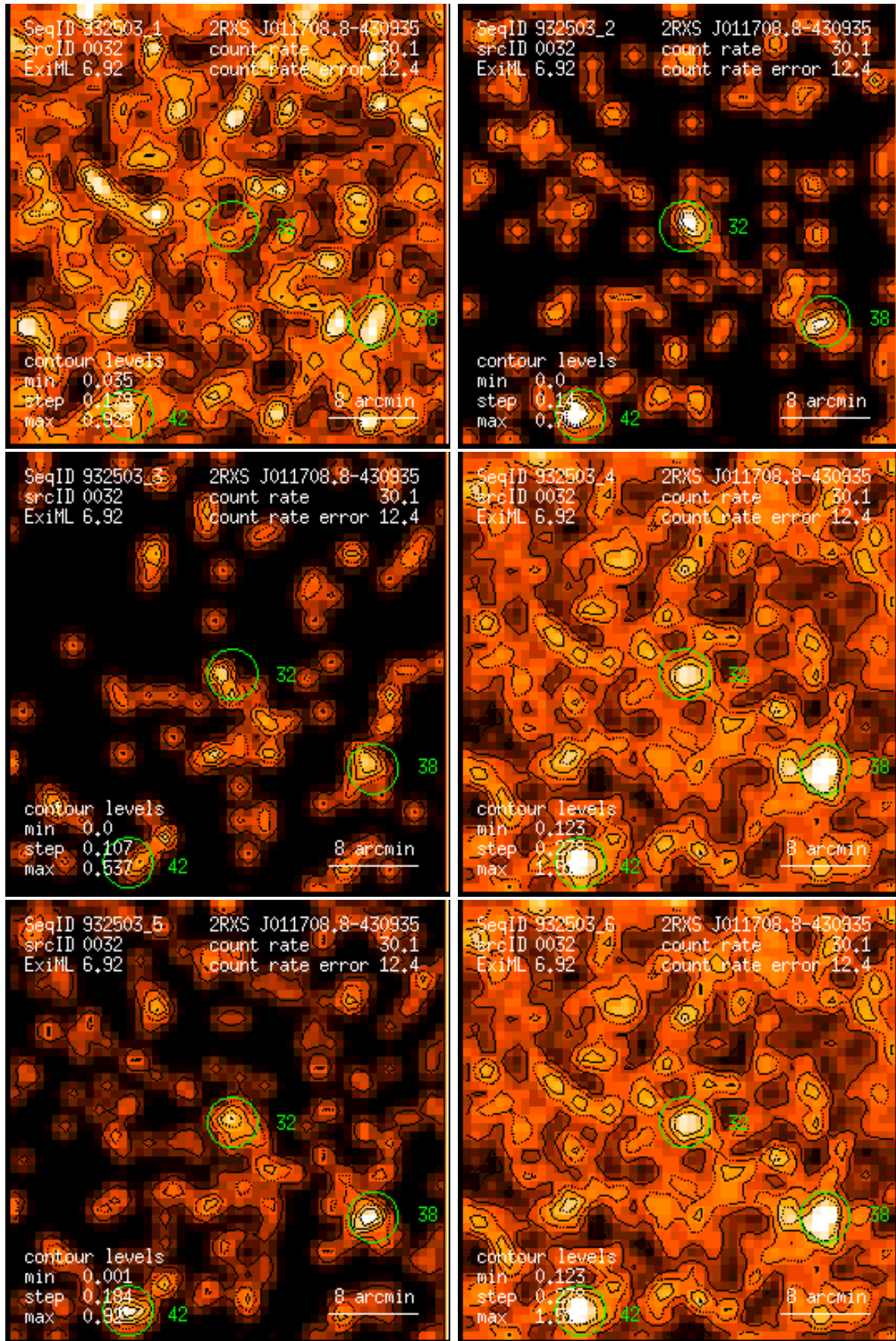
Figure 32: RASS 932503: detection 0032: band rate images, Gaussian filter: (1) PSPC channels 11 – 41, (2) 52 – 90, (3) 91 – 201, (4) 11 – 235, (5) 52 – 201, (6) 11 – 201. Broad band rates in counts/ks. Band rate contour levels in counts/ks/arcmin 2 .
