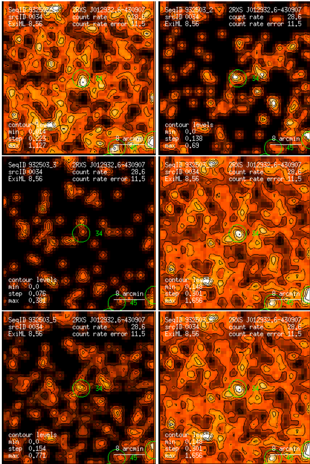
Figure 34: RASS 932503: detection 0034: band rate images, Gaussian filter: (1) PSPC channels 11 – 41, (2) 52 – 90, (3) 91 – 201, (4) 11 – 235, (5) 52 – 201, (6) 11 – 201. Broad band rates in counts/ks. Band rate contour levels in counts/ks/arcmin 2 .
