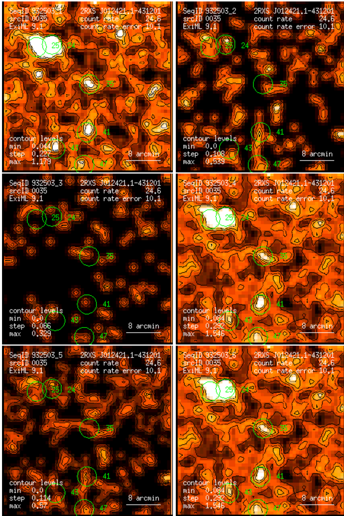
Figure 35: RASS 932503: detection 0035: band rate images, Gaussian filter: (1) PSPC channels 11 – 41, (2) 52 – 90, (3) 91 – 201, (4) 11 – 235, (5) 52 – 201, (6) 11 – 201. Broad band rates in counts/ks. Band rate contour levels in counts/ks/arcmin 2 .
