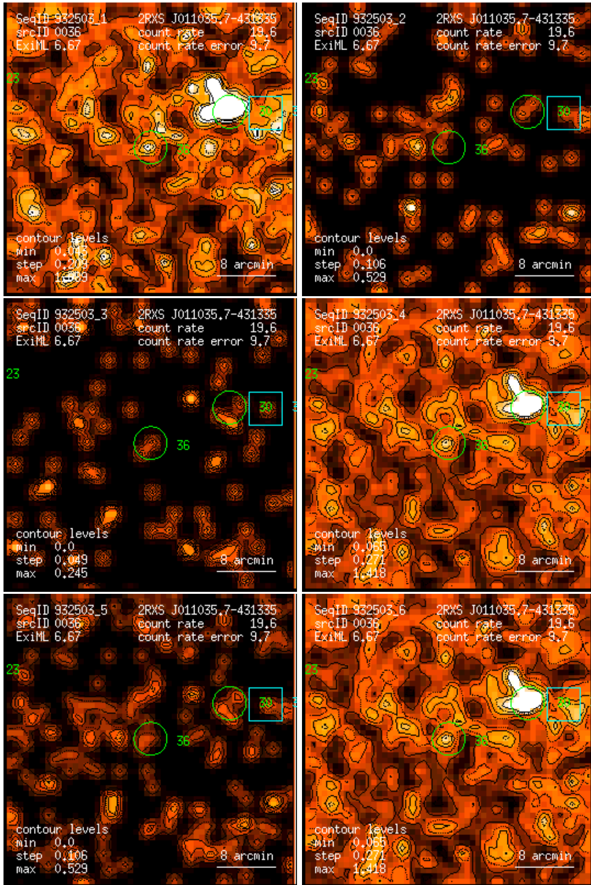
Figure 36: RASS 932503: detection 0036: band rate images, Gaussian filter: (1) PSPC channels 11 – 41, (2) 52 – 90, (3) 91 – 201, (4) 11 – 235, (5) 52 – 201, (6) 11 – 201. Broad band rates in counts/ks. Band rate contour levels in counts/ks/arcmin 2 .
