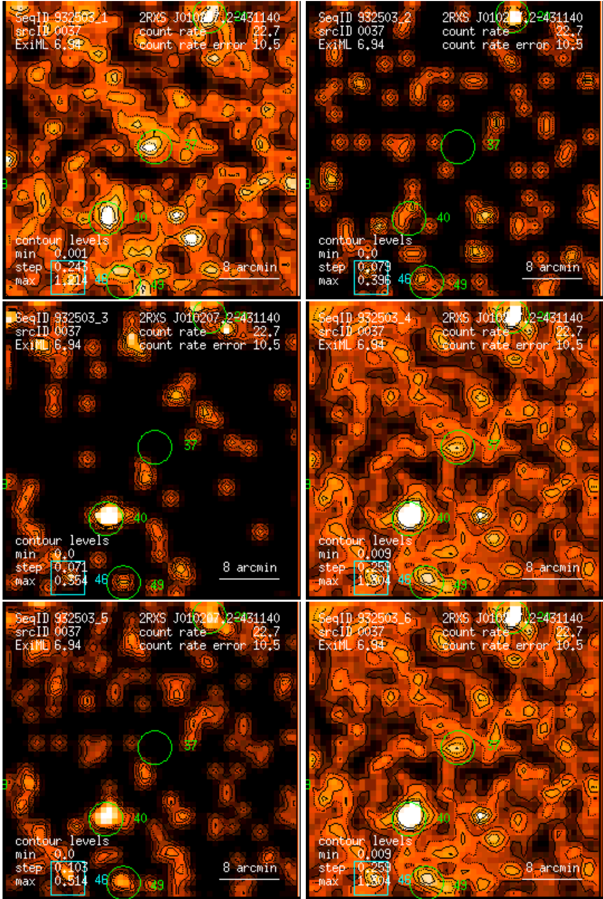
Figure 37: RASS 932503: detection 0037: band rate images, Gaussian filter: (1) PSPC channels 11 – 41, (2) 52 – 90, (3) 91 – 201, (4) 11 – 235, (5) 52 – 201, (6) 11 – 201. Broad band rates in counts/ks. Band rate contour levels in counts/ks/arcmin 2 .
