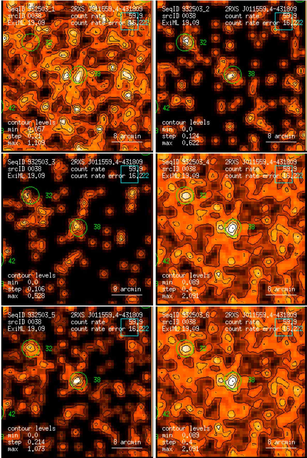
Figure 38: RASS 932503: detection 0038: band rate images, Gaussian filter: (1) PSPC channels 11 – 41, (2) 52 – 90, (3) 91 – 201, (4) 11 – 235, (5) 52 – 201, (6) 11 – 201. Broad band rates in counts/ks. Band rate contour levels in counts/ks/arcmin 2 .
