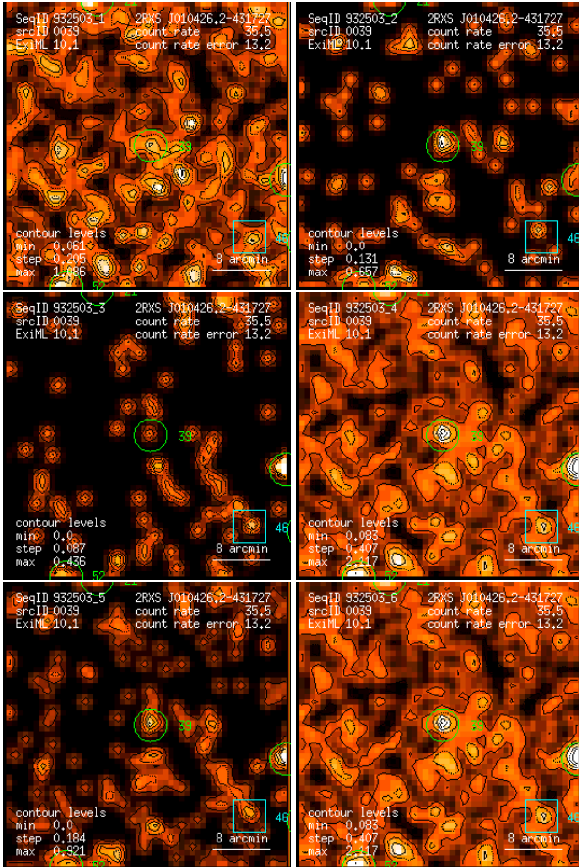
Figure 39: RASS 932503: detection 0039: band rate images, Gaussian filter: (1) PSPC channels 11 – 41, (2) 52 – 90, (3) 91 – 201, (4) 11 – 235, (5) 52 – 201, (6) 11 – 201. Broad band rates in counts/ks. Band rate contour levels in counts/ks/arcmin 2 .
