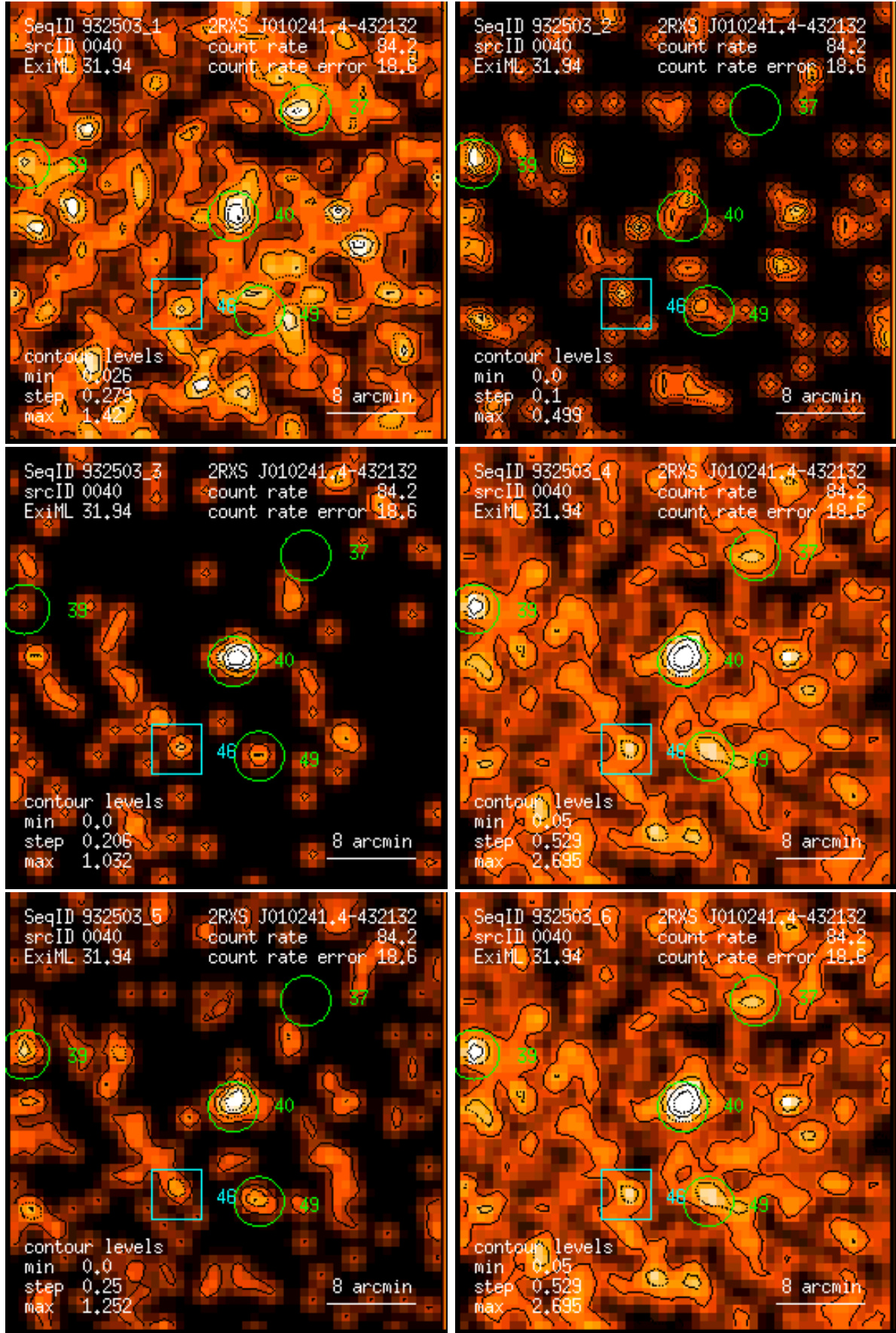
Figure 40: RASS 932503: detection 0040: band rate images, Gaussian filter: (1) PSPC channels 11 – 41, (2) 52 – 90, (3) 91 – 201, (4) 11 – 235, (5) 52 – 201, (6) 11 – 201. Broad band rates in counts/ks. Band rate contour levels in counts/ks/arcmin 2 .
