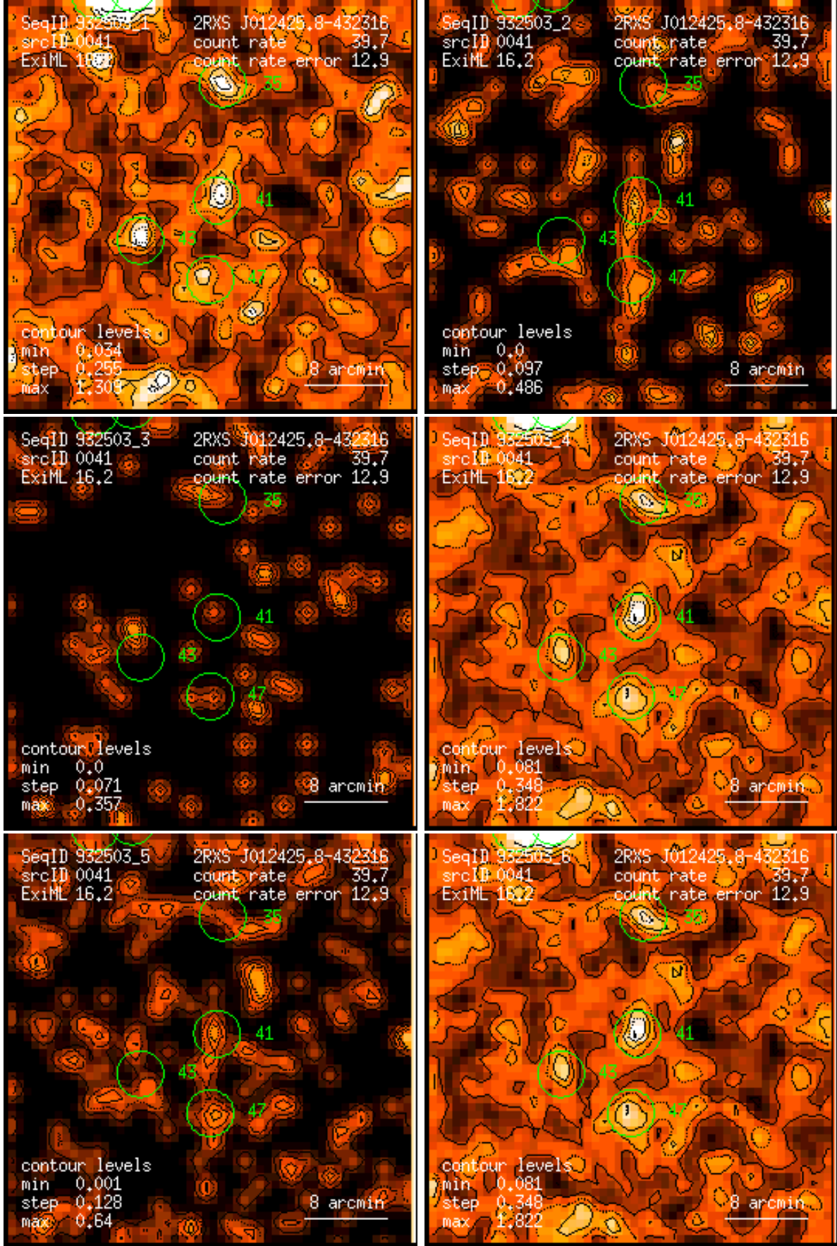
Figure 41: RASS 932503: detection 0041: band rate images, Gaussian filter: (1) PSPC channels 11 – 41, (2) 52 – 90, (3) 91 – 201, (4) 11 – 235, (5) 52 – 201, (6) 11 – 201. Broad band rates in counts/ks. Band rate contour levels in counts/ks/arcmin 2 .
