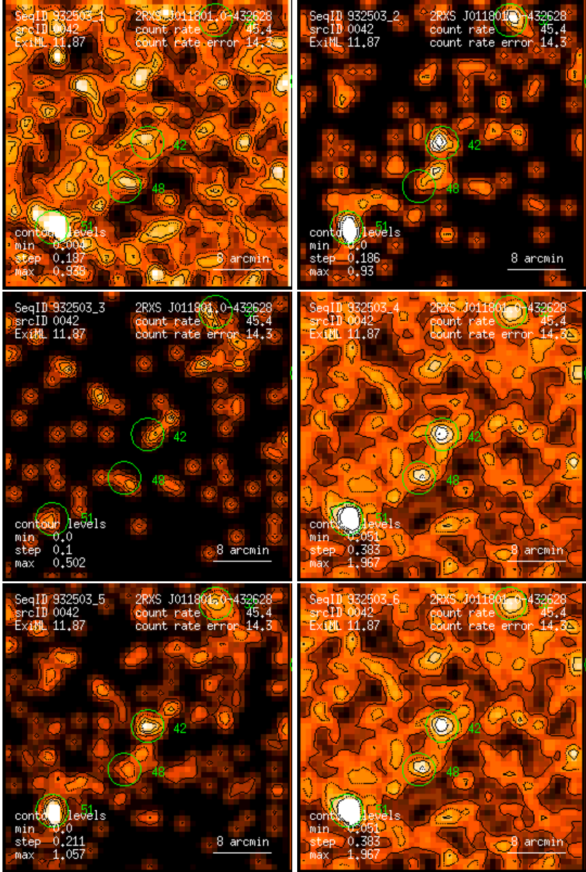
Figure 42: RASS 932503: detection 0042: band rate images, Gaussian filter: (1) PSPC channels 11 – 41, (2) 52 – 90, (3) 91 – 201, (4) 11 – 235, (5) 52 – 201, (6) 11 – 201. Broad band rates in counts/ks. Band rate contour levels in counts/ks/arcmin 2 .
