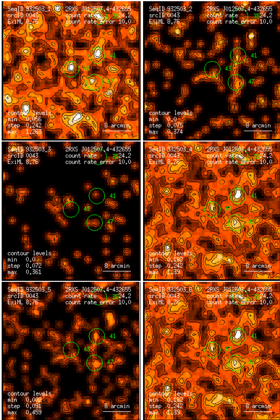
Figure 43: RASS 932503: detection 0043: band rate images, Gaussian filter: (1) PSPC channels 11 – 41, (2) 52 – 90, (3) 91 – 201, (4) 11 – 235, (5) 52 – 201, (6) 11 – 201. Broad band rates in counts/ks. Band rate contour levels in counts/ks/arcmin 2 .
