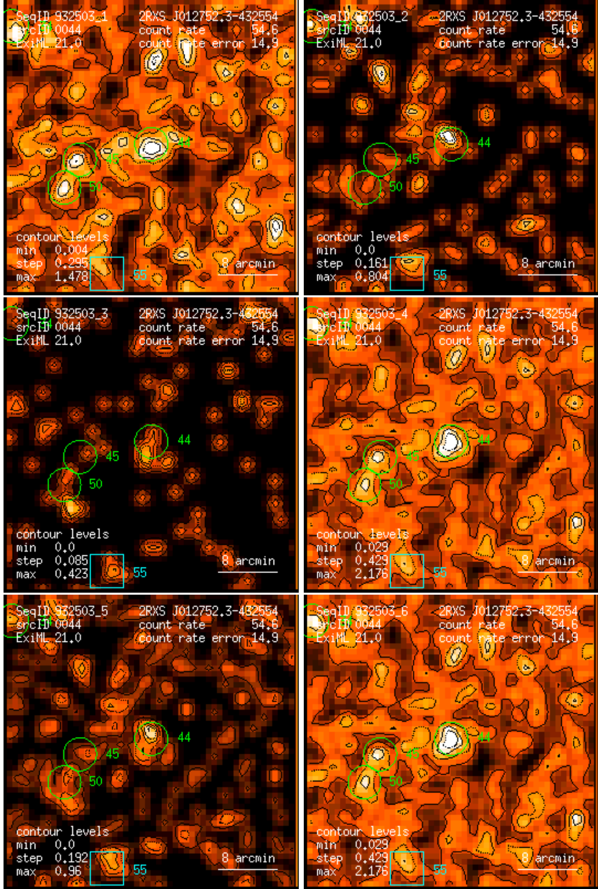
Figure 44: RASS 932503: detection 0044: band rate images, Gaussian filter: (1) PSPC channels 11 – 41, (2) 52 – 90, (3) 91 – 201, (4) 11 – 235, (5) 52 – 201, (6) 11 – 201. Broad band rates in counts/ks. Band rate contour levels in counts/ks/arcmin 2 .
