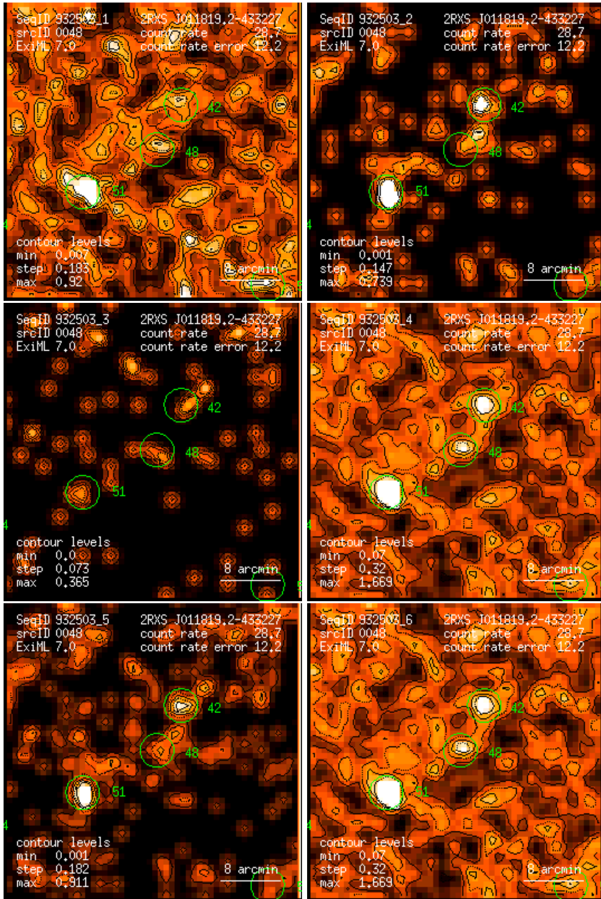
Figure 48: RASS 932503: detection 0048: band rate images, Gaussian filter: (1) PSPC channels 11 – 41, (2) 52 – 90, (3) 91 – 201, (4) 11 – 235, (5) 52 – 201, (6) 11 – 201. Broad band rates in counts/ks. Band rate contour levels in counts/ks/arcmin 2 .
