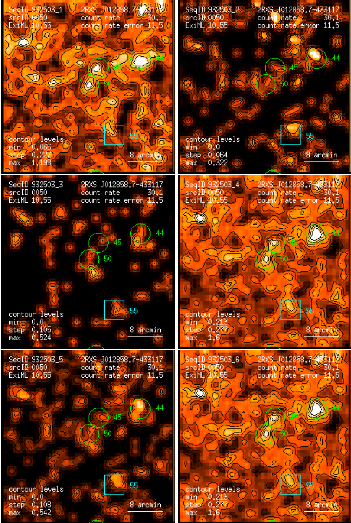
Figure 50: RASS 932503: detection 0050: band rate images, Gaussian filter: (1) PSPC channels 11 – 41, (2) 52 – 90, (3) 91 – 201, (4) 11 – 235, (5) 52 – 201, (6) 11 – 201. Broad band rates in counts/ks. Band rate contour levels in counts/ks/arcmin 2 .
