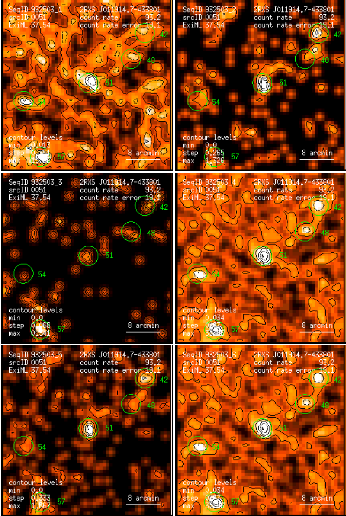
Figure 51: RASS 932503: detection 0051: band rate images, Gaussian filter: (1) PSPC channels 11 – 41, (2) 52 – 90, (3) 91 – 201, (4) 11 – 235, (5) 52 – 201, (6) 11 – 201. Broad band rates in counts/ks. Band rate contour levels in counts/ks/arcmin 2 .
