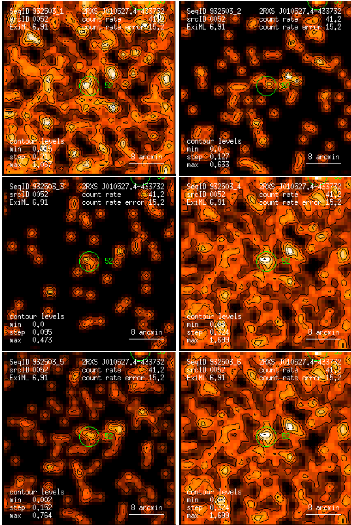
Figure 52: RASS 932503: detection 0052: band rate images, Gaussian filter: (1) PSPC channels 11 – 41, (2) 52 – 90, (3) 91 – 201, (4) 11 – 235, (5) 52 – 201, (6) 11 – 201. Broad band rates in counts/ks. Band rate contour levels in counts/ks/arcmin 2 .
